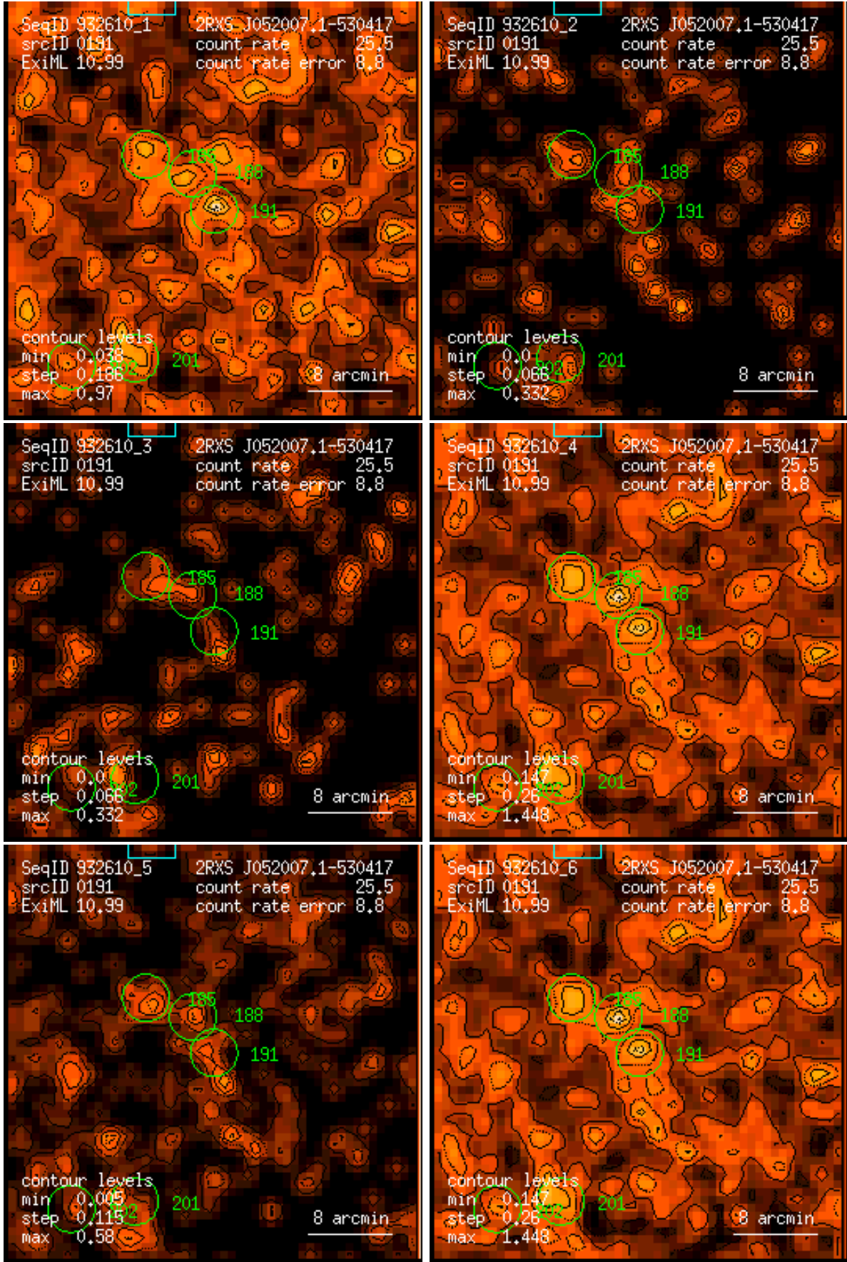
Figure 191: RASS 932610: detection 0191: band rate images, Gaussian filter: (1) PSPC channels 11 – 41, (2) 52 – 90, (3) 91 – 201, (4) 11 – 235, (5) 52 – 201, (6) 11 – 201. Broad band rates in counts/ks. Band rate contour levels in counts/ks/arcmin 2 .
