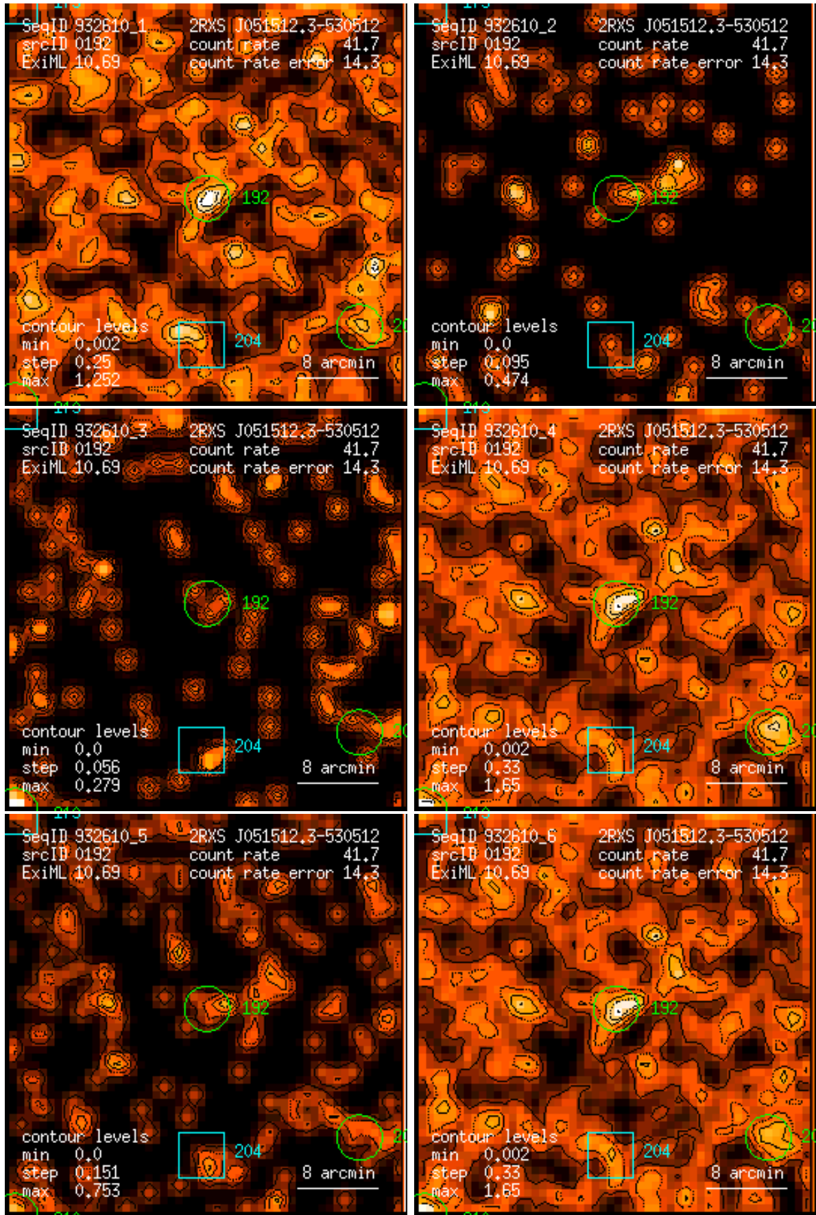
Figure 192: RASS 932610: detection 0192: band rate images, Gaussian filter: (1) PSPC channels 11 – 41, (2) 52 – 90, (3) 91 – 201, (4) 11 – 235, (5) 52 – 201, (6) 11 – 201. Broad band rates in counts/ks. Band rate contour levels in counts/ks/arcmin 2 .
