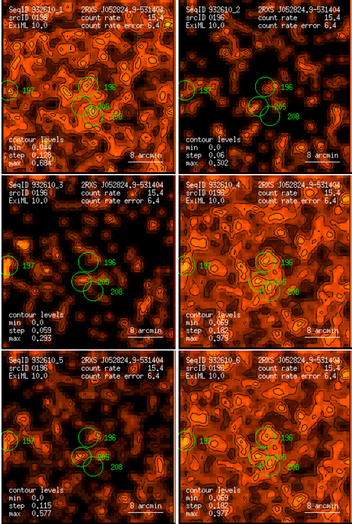
Figure 196: RASS 932610: detection 0196: band rate images, Gaussian filter: (1) PSPC channels 11 – 41, (2) 52 – 90, (3) 91 – 201, (4) 11 – 235, (5) 52 – 201, (6) 11 – 201. Broad band rates in counts/ks. Band rate contour levels in counts/ks/arcmin 2 .
