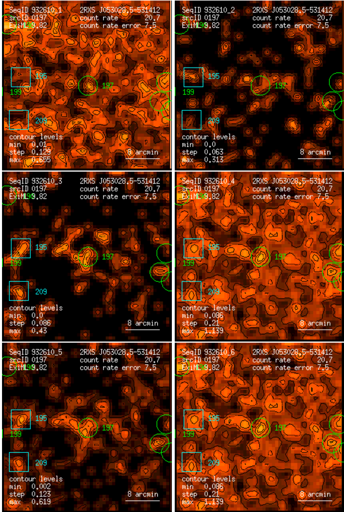
Figure 197: RASS 932610: detection 0197: band rate images, Gaussian filter: (1) PSPC channels 11 – 41, (2) 52 – 90, (3) 91 – 201, (4) 11 – 235, (5) 52 – 201, (6) 11 – 201. Broad band rates in counts/ks. Band rate contour levels in counts/ks/arcmin 2 .
