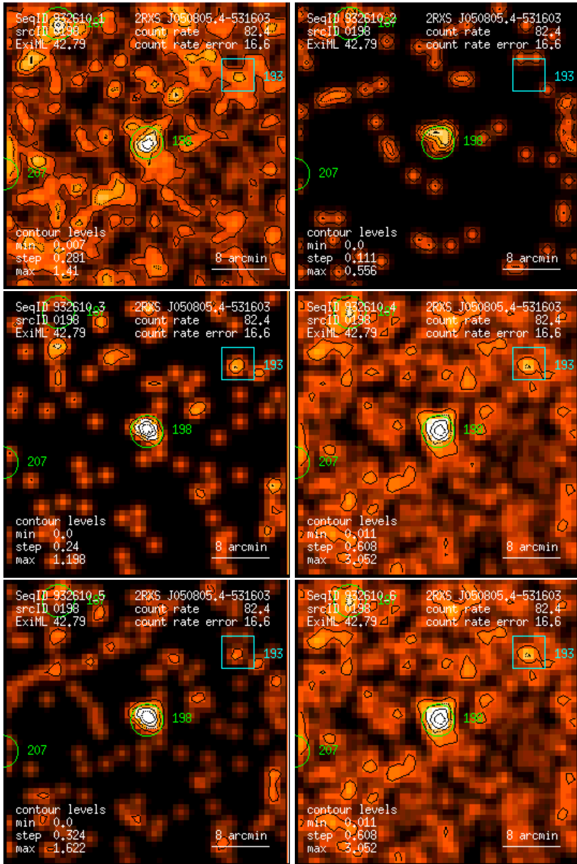
Figure 198: RASS 932610: detection 0198: band rate images, Gaussian filter: (1) PSPC channels 11 – 41, (2) 52 – 90, (3) 91 – 201, (4) 11 – 235, (5) 52 – 201, (6) 11 – 201. Broad band rates in counts/ks. Band rate contour levels in counts/ks/arcmin 2 .
