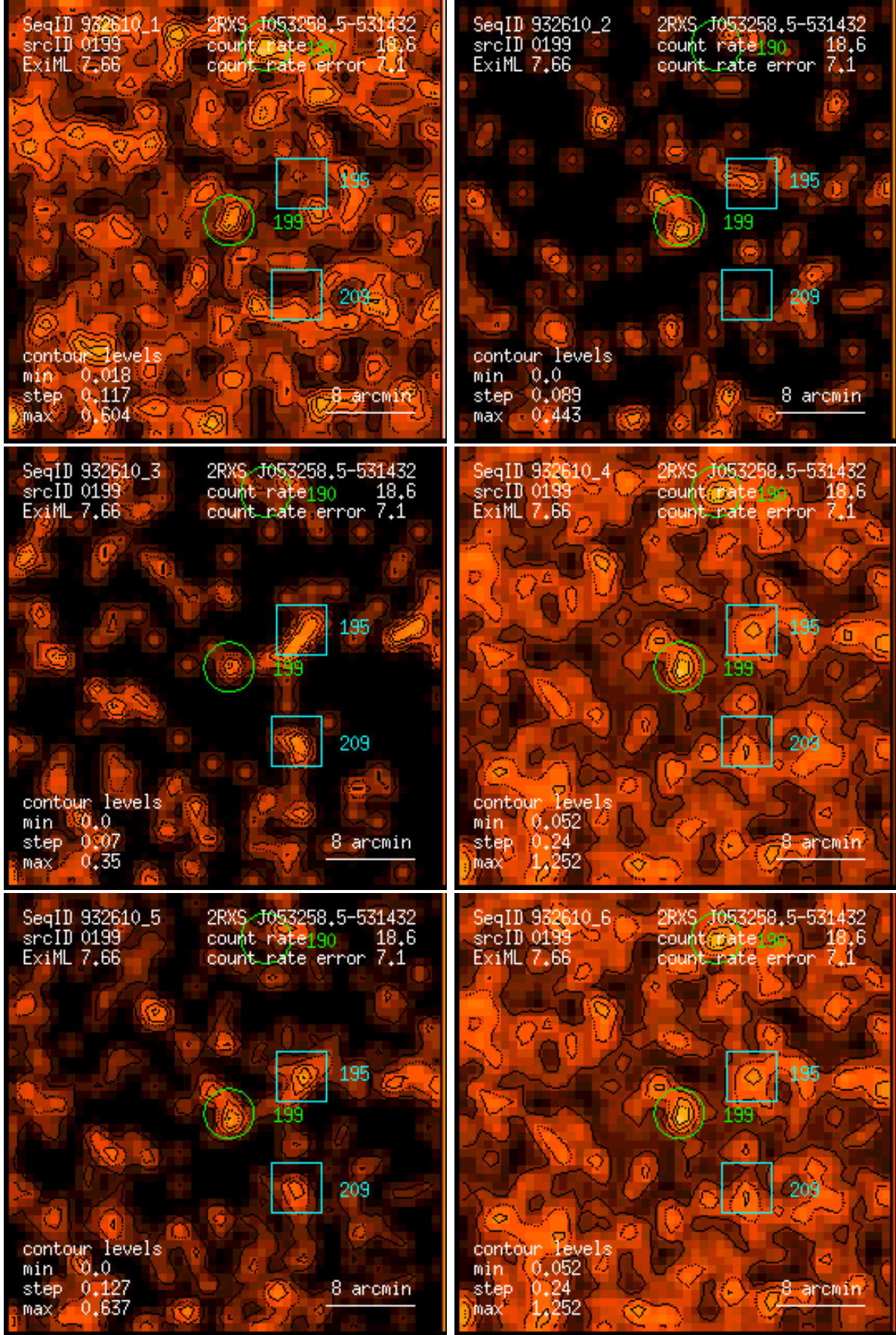
Figure 199: RASS 932610: detection 0199: band rate images, Gaussian filter: (1) PSPC channels 11 – 41, (2) 52 – 90, (3) 91 – 201, (4) 11 – 235, (5) 52 – 201, (6) 11 – 201. Broad band rates in counts/ks. Band rate contour levels in counts/ks/arcmin 2 .
