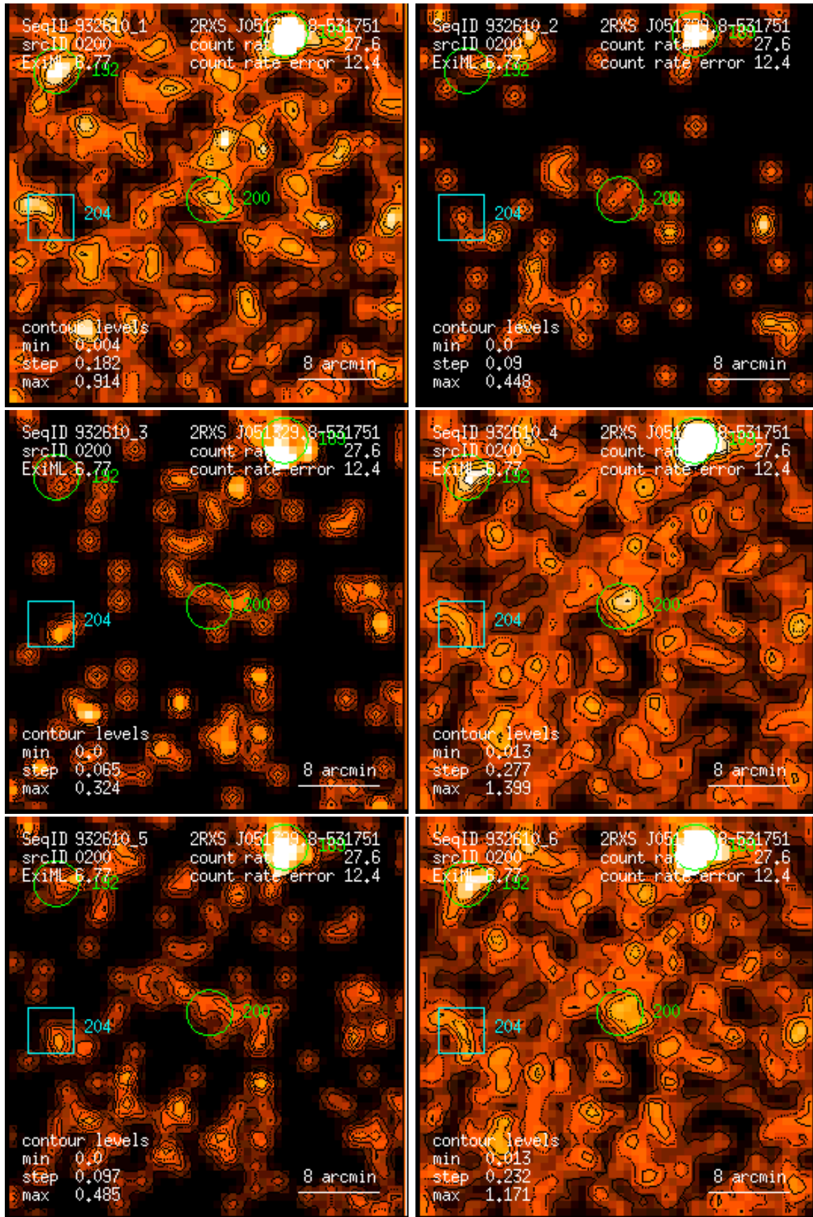
Figure 200: RASS 932610: detection 0200: band rate images, Gaussian filter: (1) PSPC channels 11 – 41, (2) 52 – 90, (3) 91 – 201, (4) 11 – 235, (5) 52 – 201, (6) 11 – 201. Broad band rates in counts/ks. Band rate contour levels in counts/ks/arcmin 2 .
