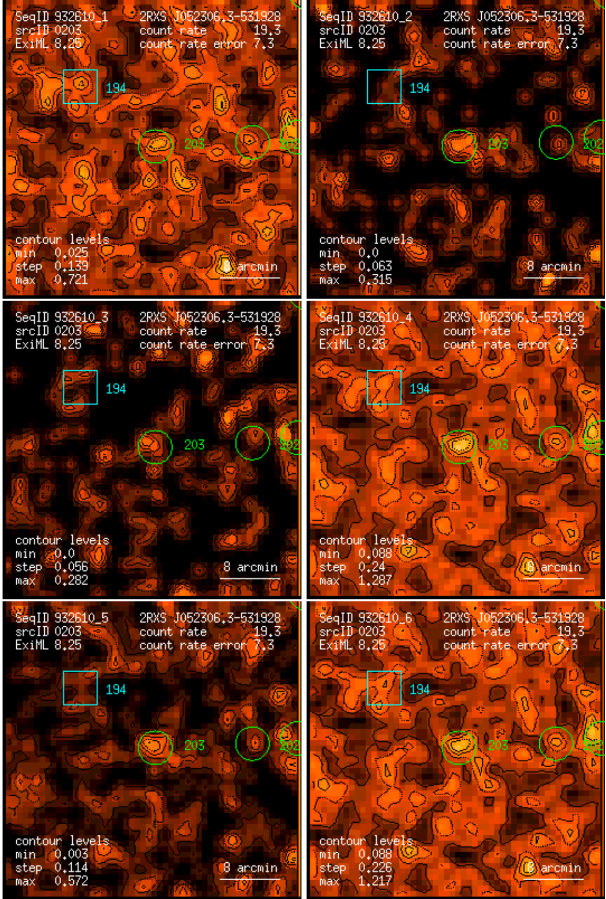
Figure 203: RASS 932610: detection 0203: band rate images, Gaussian filter: (1) PSPC channels 11 – 41, (2) 52 – 90, (3) 91 – 201, (4) 11 – 235, (5) 52 – 201, (6) 11 – 201. Broad band rates in counts/ks. Band rate contour levels in counts/ks/arcmin 2 .
