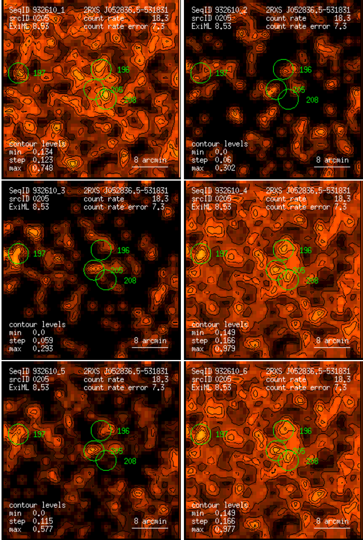
Figure 205: RASS 932610: detection 0205: band rate images, Gaussian filter: (1) PSPC channels 11 – 41, (2) 52 – 90, (3) 91 – 201, (4) 11 – 235, (5) 52 – 201, (6) 11 – 201. Broad band rates in counts/ks. Band rate contour levels in counts/ks/arcmin 2 .
