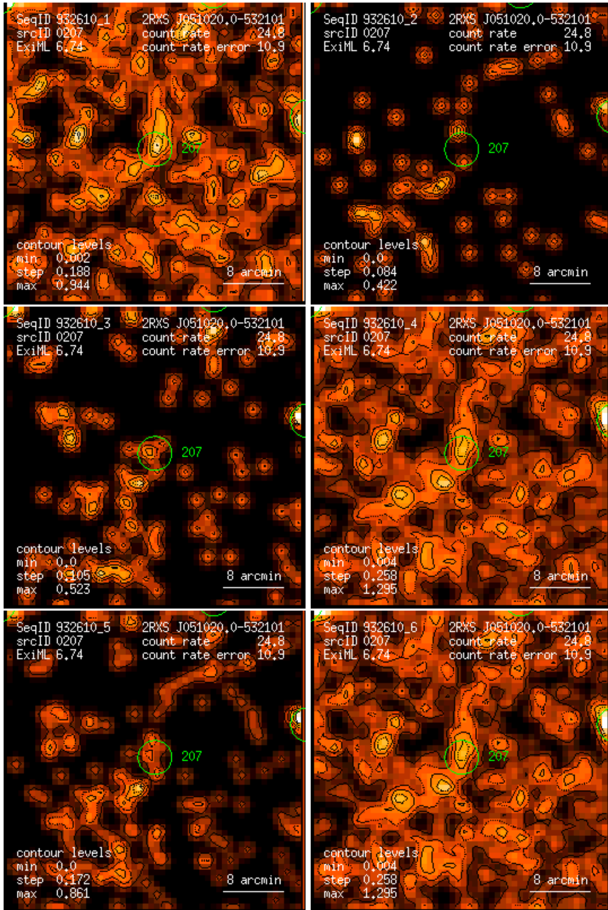
Figure 207: RASS 932610: detection 0207: band rate images, Gaussian filter: (1) PSPC channels 11 – 41, (2) 52 – 90, (3) 91 – 201, (4) 11 – 235, (5) 52 – 201, (6) 11 – 201. Broad band rates in counts/ks. Band rate contour levels in counts/ks/arcmin 2 .
