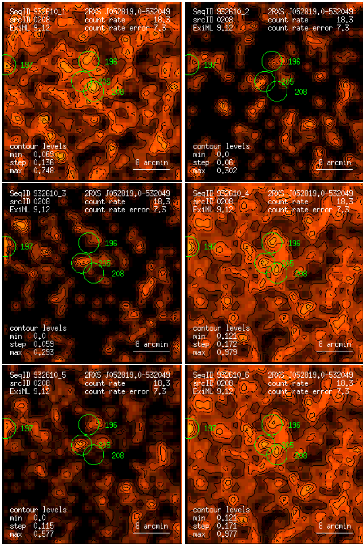
Figure 208: RASS 932610: detection 0208: band rate images, Gaussian filter: (1) PSPC channels 11 – 41, (2) 52 – 90, (3) 91 – 201, (4) 11 – 235, (5) 52 – 201, (6) 11 – 201. Broad band rates in counts/ks. Band rate contour levels in counts/ks/arcmin 2 .
