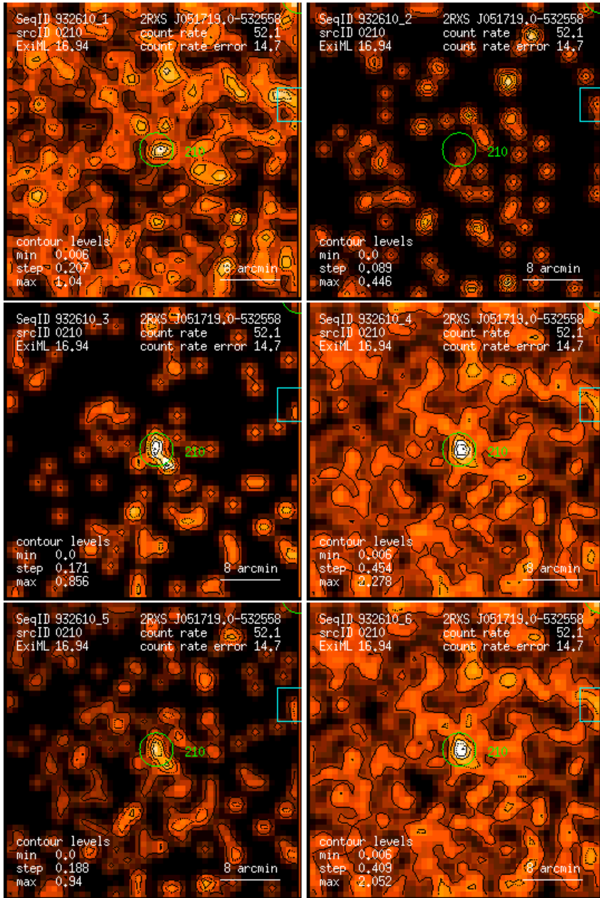
Figure 210: RASS 932610: detection 0210: band rate images, Gaussian filter: (1) PSPC channels 11 – 41, (2) 52 – 90, (3) 91 – 201, (4) 11 – 235, (5) 52 – 201, (6) 11 – 201. Broad band rates in counts/ks. Band rate contour levels in counts/ks/arcmin 2 .
