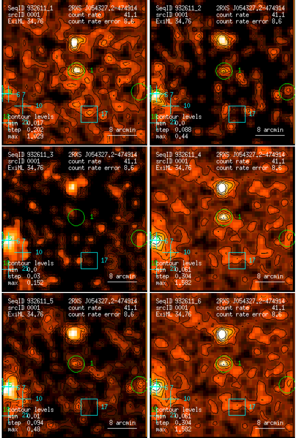
Figure 1: RASS 932611: detection 0001: band rate images, Gaussian filter: (1) PSPC channels 11 – 41, (2) 52 – 90, (3) 91 – 201, (4) 11 – 235, (5) 52 – 201, (6) 11 – 201. Broad band rates in counts/ks. Band rate contour levels in counts/ks/arcmin 2 .
