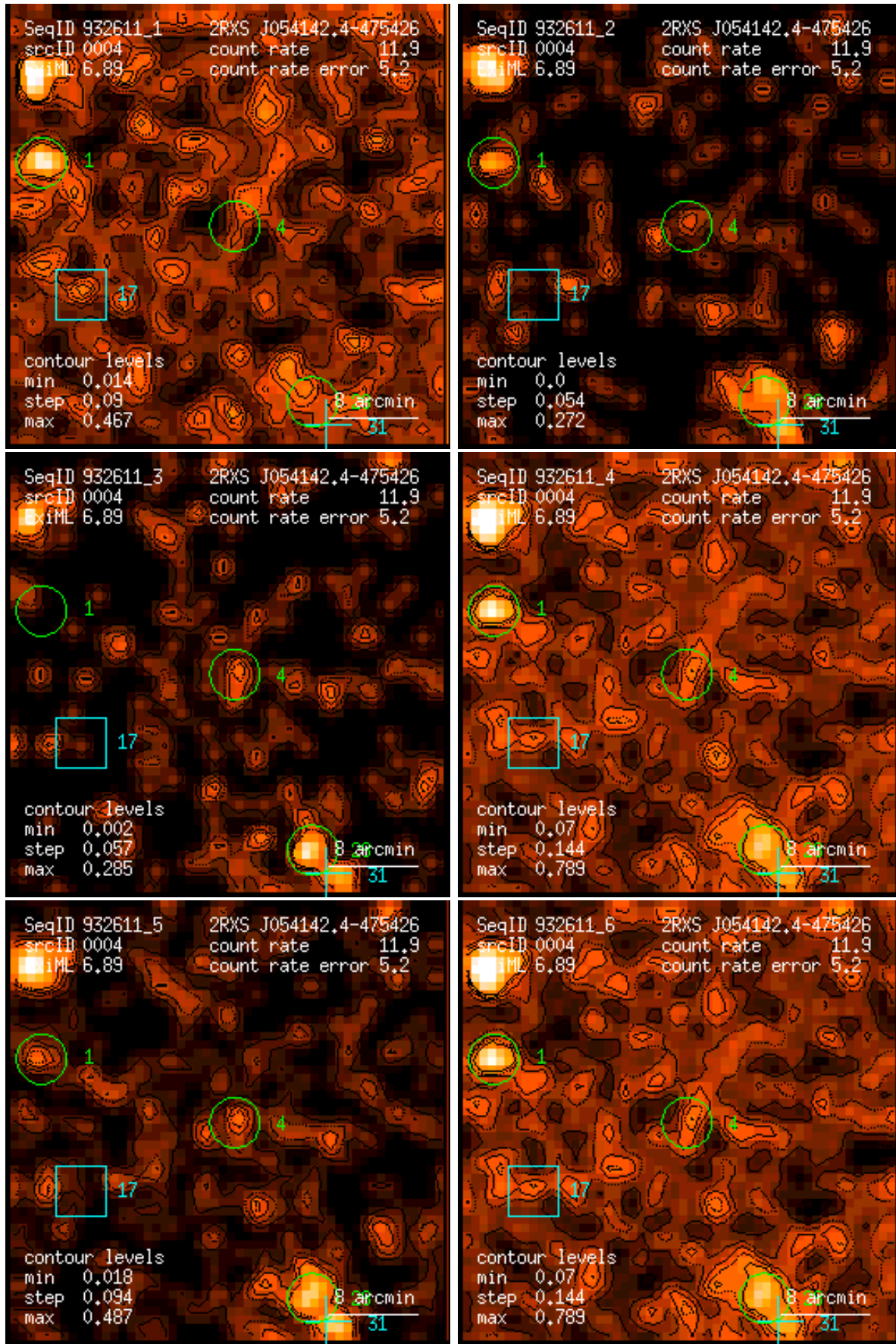
Figure 4: RASS 932611: detection 0004: band rate images, Gaussian filter: (1) PSPC channels 11 – 41, (2) 52 – 90, (3) 91 – 201, (4) 11 – 235, (5) 52 – 201, (6) 11 – 201. Broad band rates in counts/ks. Band rate contour levels in counts/ks/arcmin 2 .
