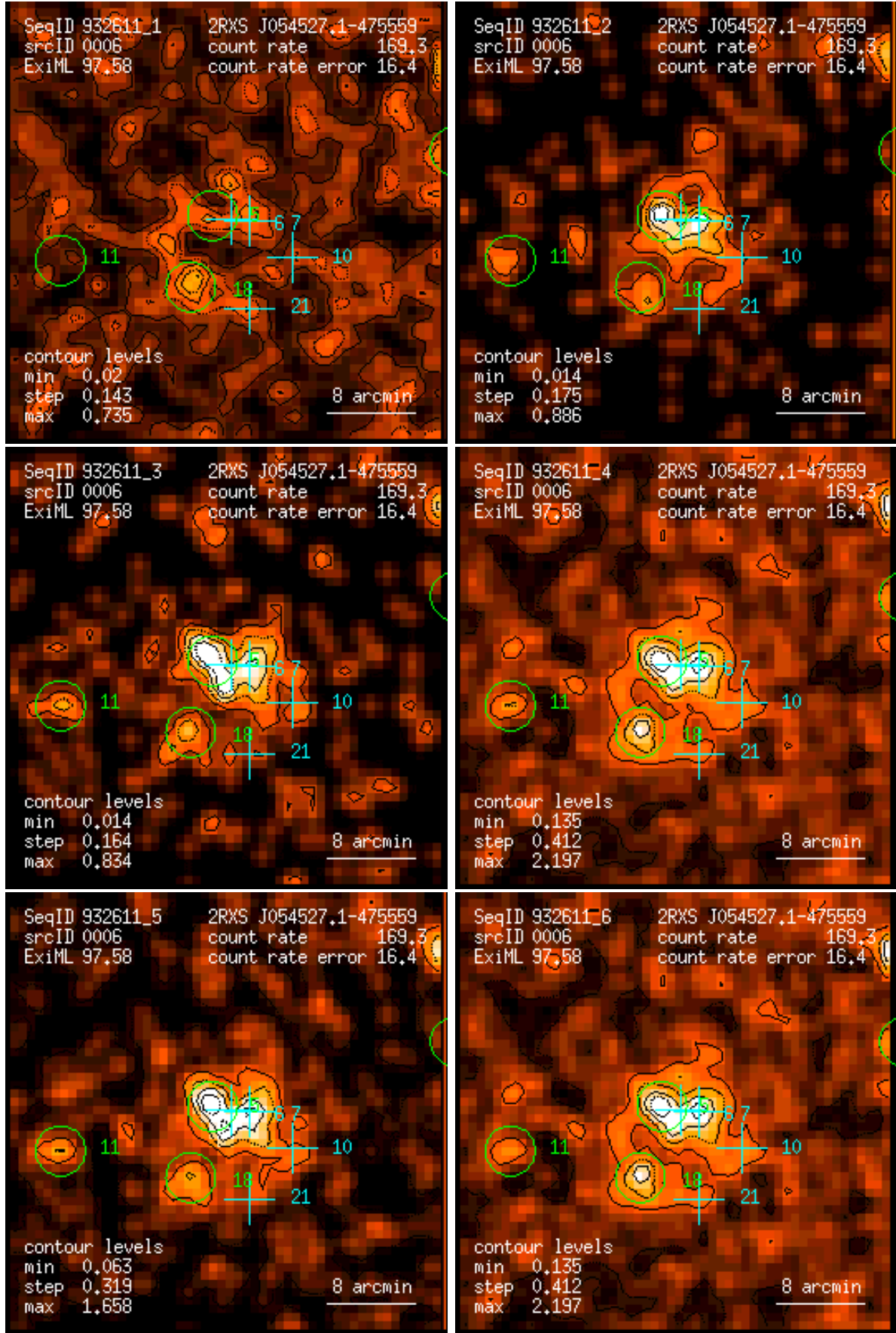
Figure 6: RASS 932611: detection 0006: band rate images, Gaussian filter: (1) PSPC channels 11 – 41, (2) 52 – 90, (3) 91 – 201, (4) 11 – 235, (5) 52 – 201, (6) 11 – 201. Broad band rates in counts/ks. Band rate contour levels in counts/ks/arcmin 2 .
