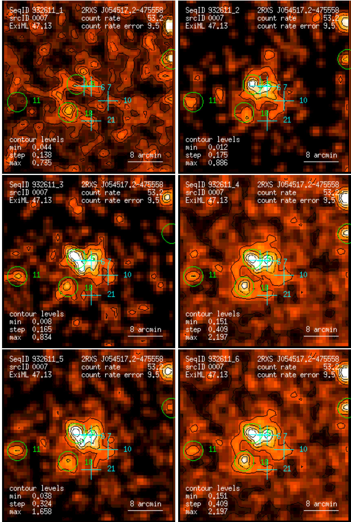
Figure 7: RASS 932611: detection 0007: band rate images, Gaussian filter: (1) PSPC channels 11 – 41, (2) 52 – 90, (3) 91 – 201, (4) 11 – 235, (5) 52 – 201, (6) 11 – 201. Broad band rates in counts/ks. Band rate contour levels in counts/ks/arcmin 2 .
