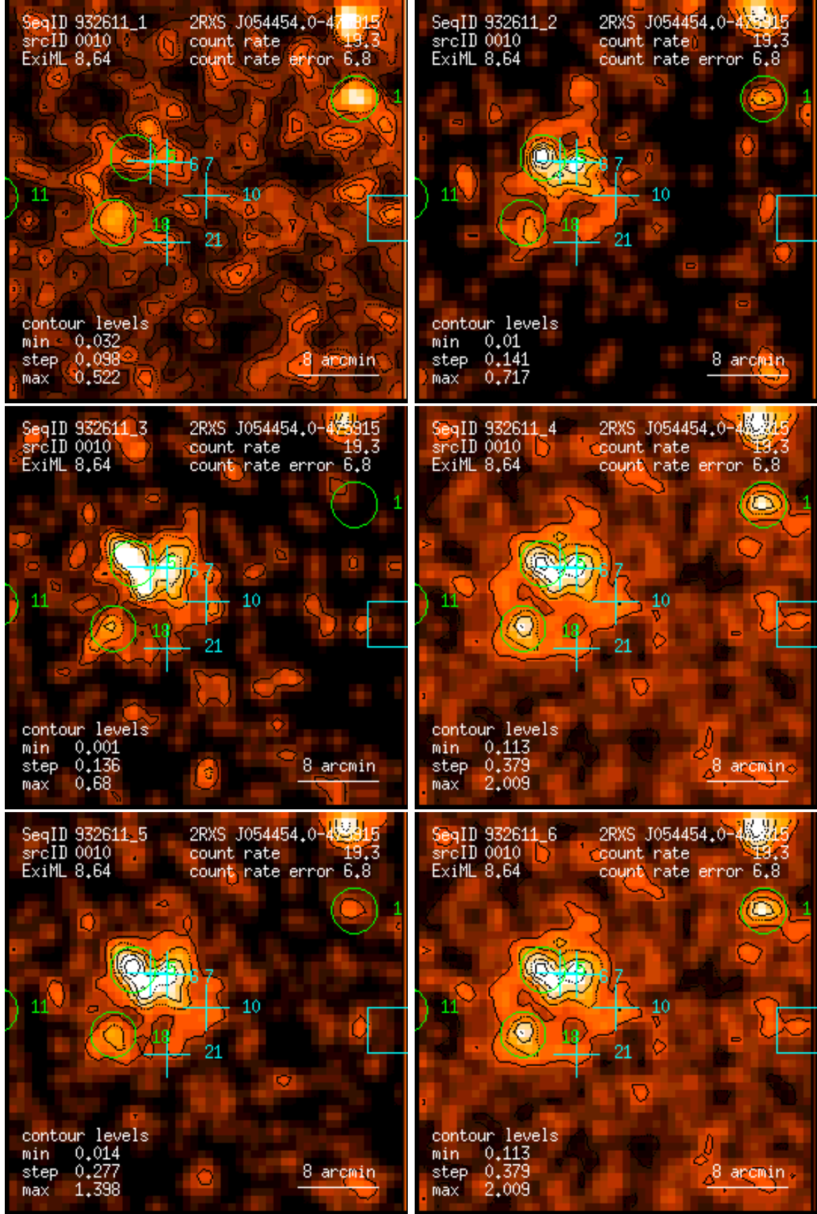
Figure 10: RASS 932611: detection 0010: band rate images, Gaussian filter: (1) PSPC channels 11 – 41, (2) 52 – 90, (3) 91 – 201, (4) 11 – 235, (5) 52 – 201, (6) 11 – 201. Broad band rates in counts/ks. Band rate contour levels in counts/ks/arcmin 2 .
