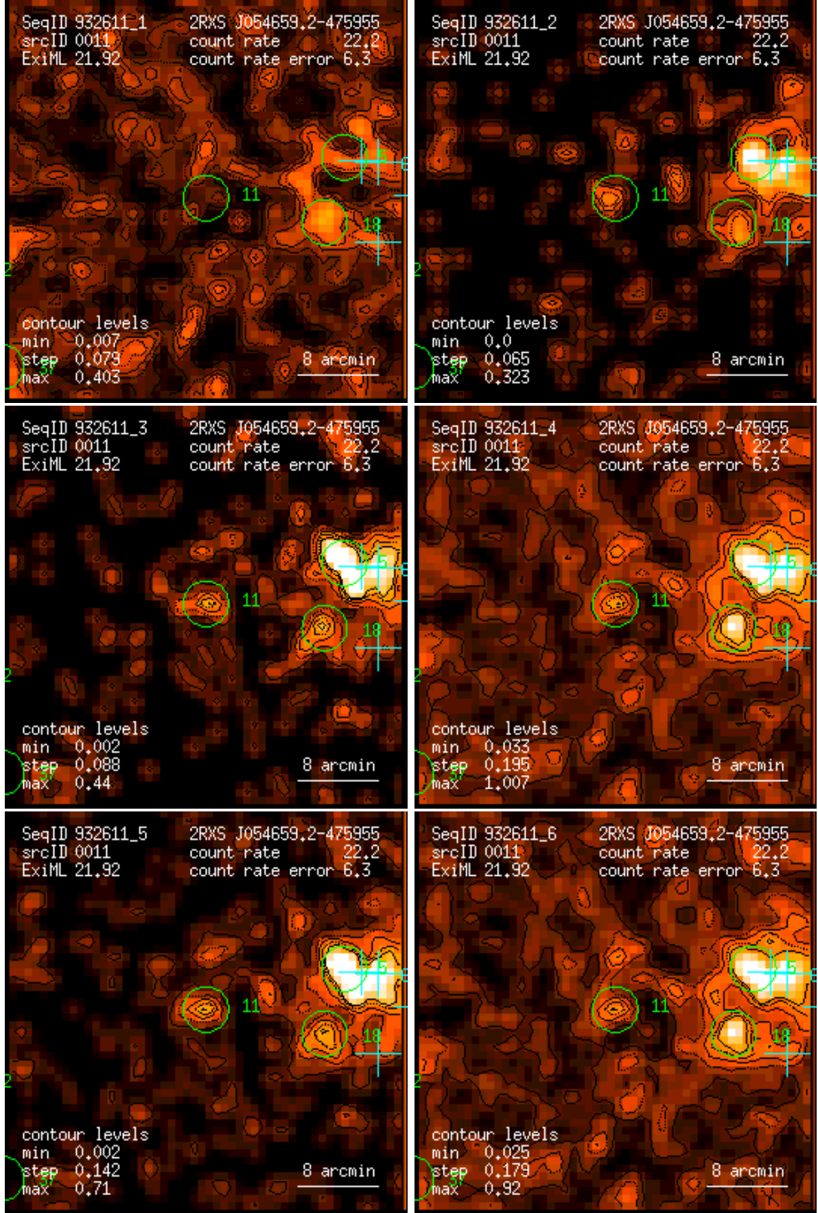
Figure 11: RASS 932611: detection 0011: band rate images, Gaussian filter: (1) PSPC channels 11 – 41, (2) 52 – 90, (3) 91 – 201, (4) 11 – 235, (5) 52 – 201, (6) 11 – 201. Broad band rates in counts/ks. Band rate contour levels in counts/ks/arcmin 2 .
