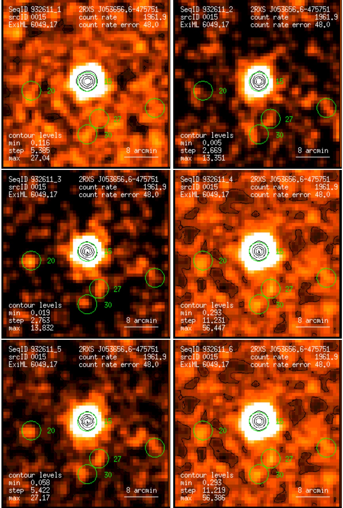
Figure 15: RASS 932611: detection 0015: band rate images, Gaussian filter: (1) PSPC channels 11 – 41, (2) 52 – 90, (3) 91 – 201, (4) 11 – 235, (5) 52 – 201, (6) 11 – 201. Broad band rates in counts/ks. Band rate contour levels in counts/ks/arcmin 2 .
