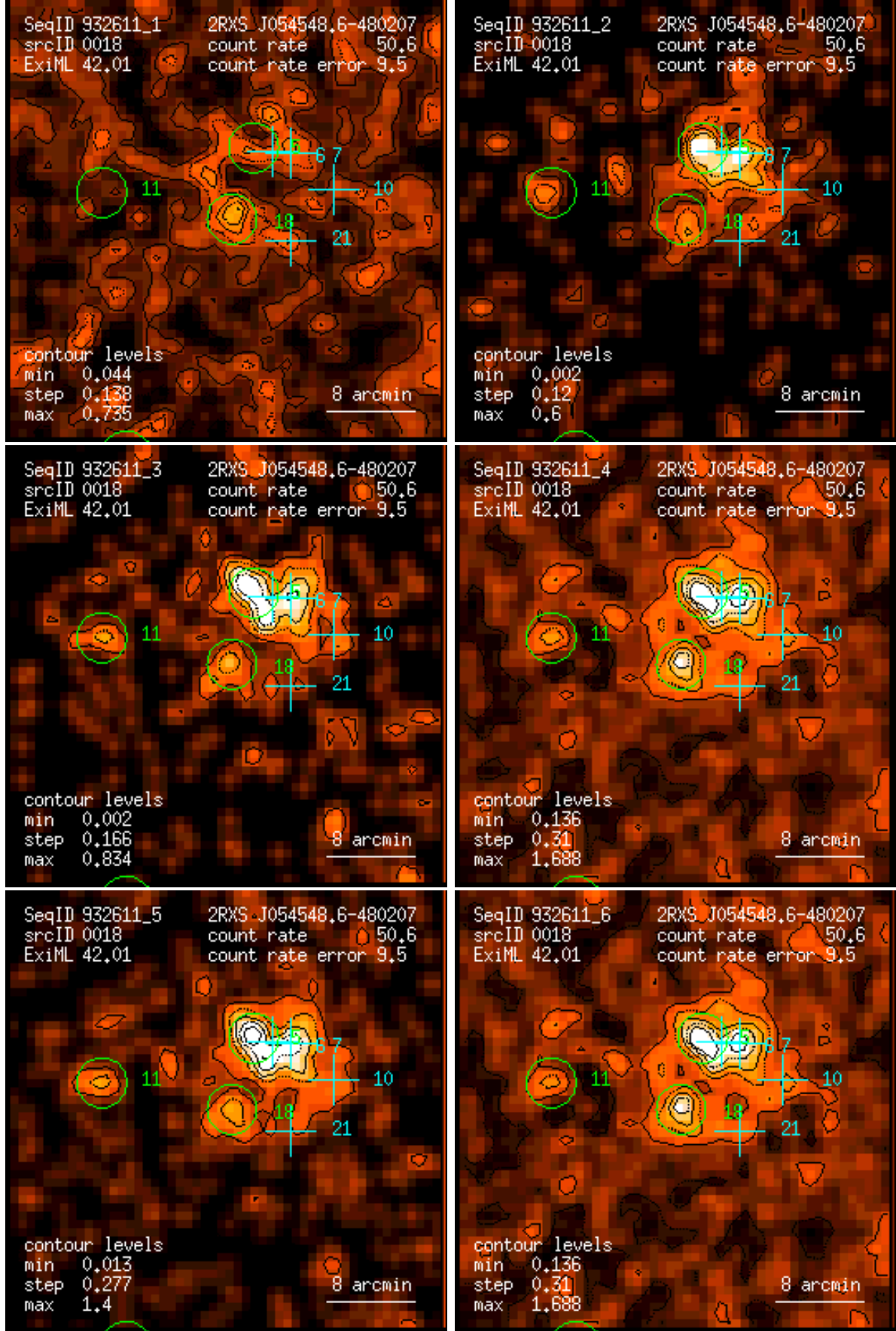
Figure 18: RASS 932611: detection 0018: band rate images, Gaussian filter: (1) PSPC channels 11 – 41, (2) 52 – 90, (3) 91 – 201, (4) 11 – 235, (5) 52 – 201, (6) 11 – 201. Broad band rates in counts/ks. Band rate contour levels in counts/ks/arcmin 2 .
