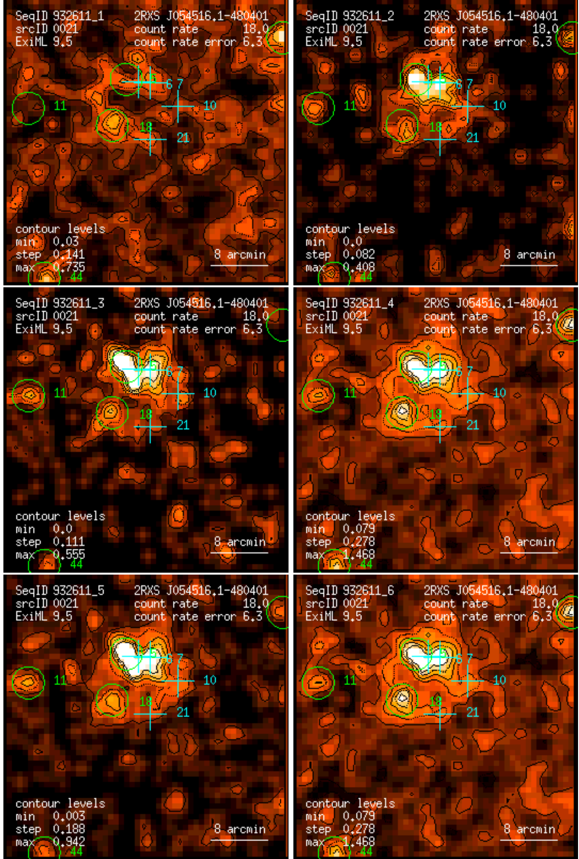
Figure 21: RASS 932611: detection 0021: band rate images, Gaussian filter: (1) PSPC channels 11 – 41, (2) 52 – 90, (3) 91 – 201, (4) 11 – 235, (5) 52 – 201, (6) 11 – 201. Broad band rates in counts/ks. Band rate contour levels in counts/ks/arcmin 2 .
