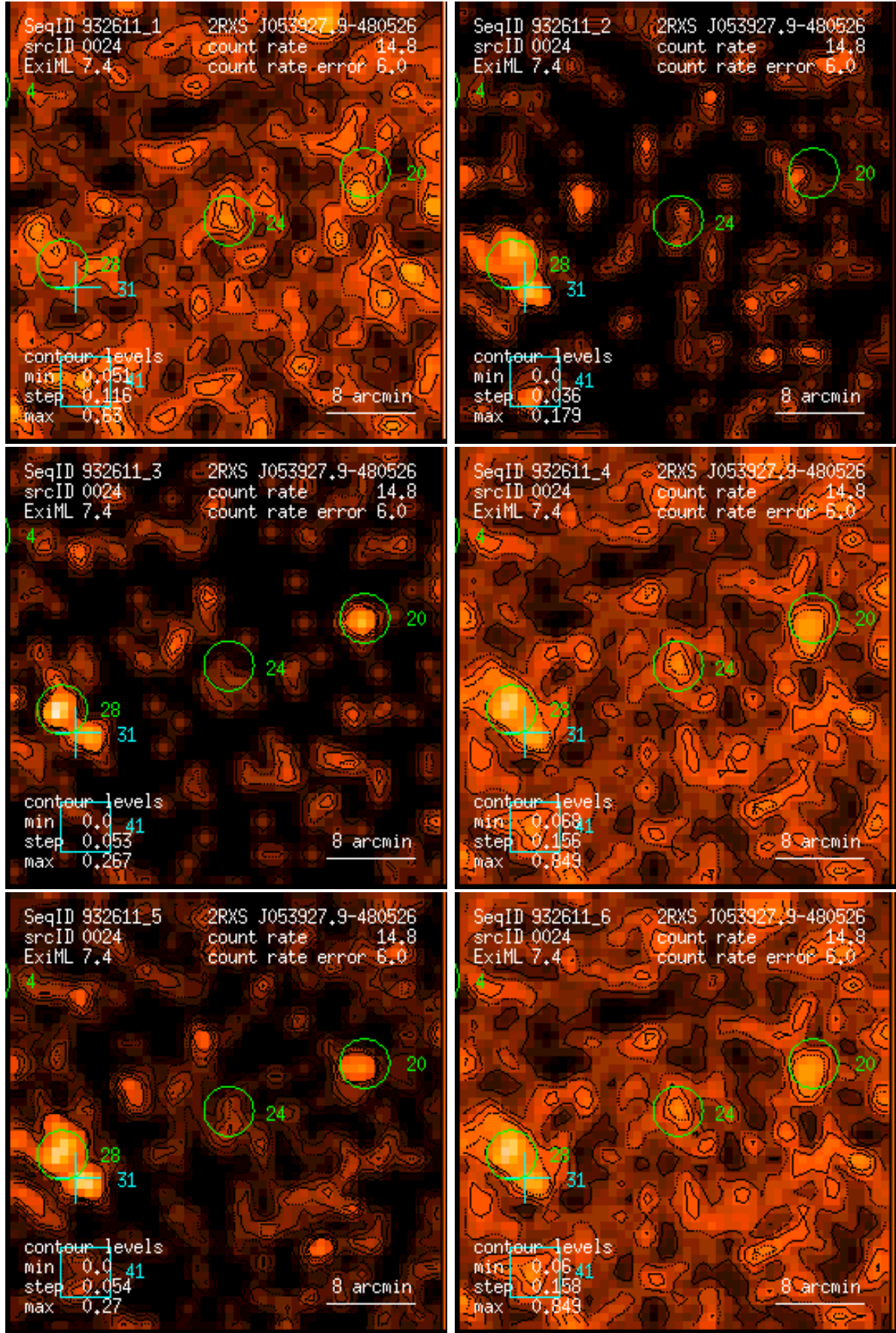
Figure 24: RASS 932611: detection 0024: band rate images, Gaussian filter: (1) PSPC channels 11 – 41, (2) 52 – 90, (3) 91 – 201, (4) 11 – 235, (5) 52 – 201, (6) 11 – 201. Broad band rates in counts/ks. Band rate contour levels in counts/ks/arcmin 2 .
