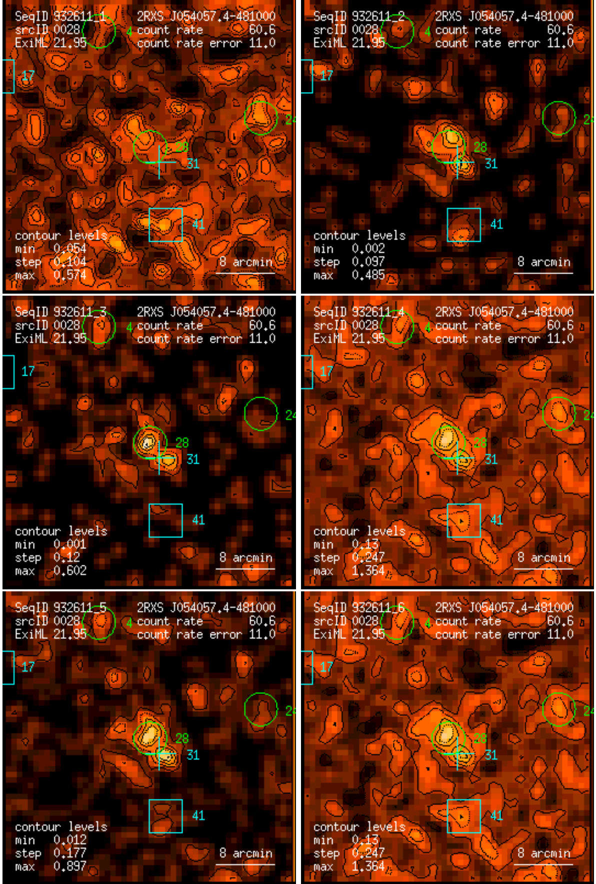
Figure 28: RASS 932611: detection 0028: band rate images, Gaussian filter: (1) PSPC channels 11 – 41, (2) 52 – 90, (3) 91 – 201, (4) 11 – 235, (5) 52 – 201, (6) 11 – 201. Broad band rates in counts/ks. Band rate contour levels in counts/ks/arcmin 2 .
