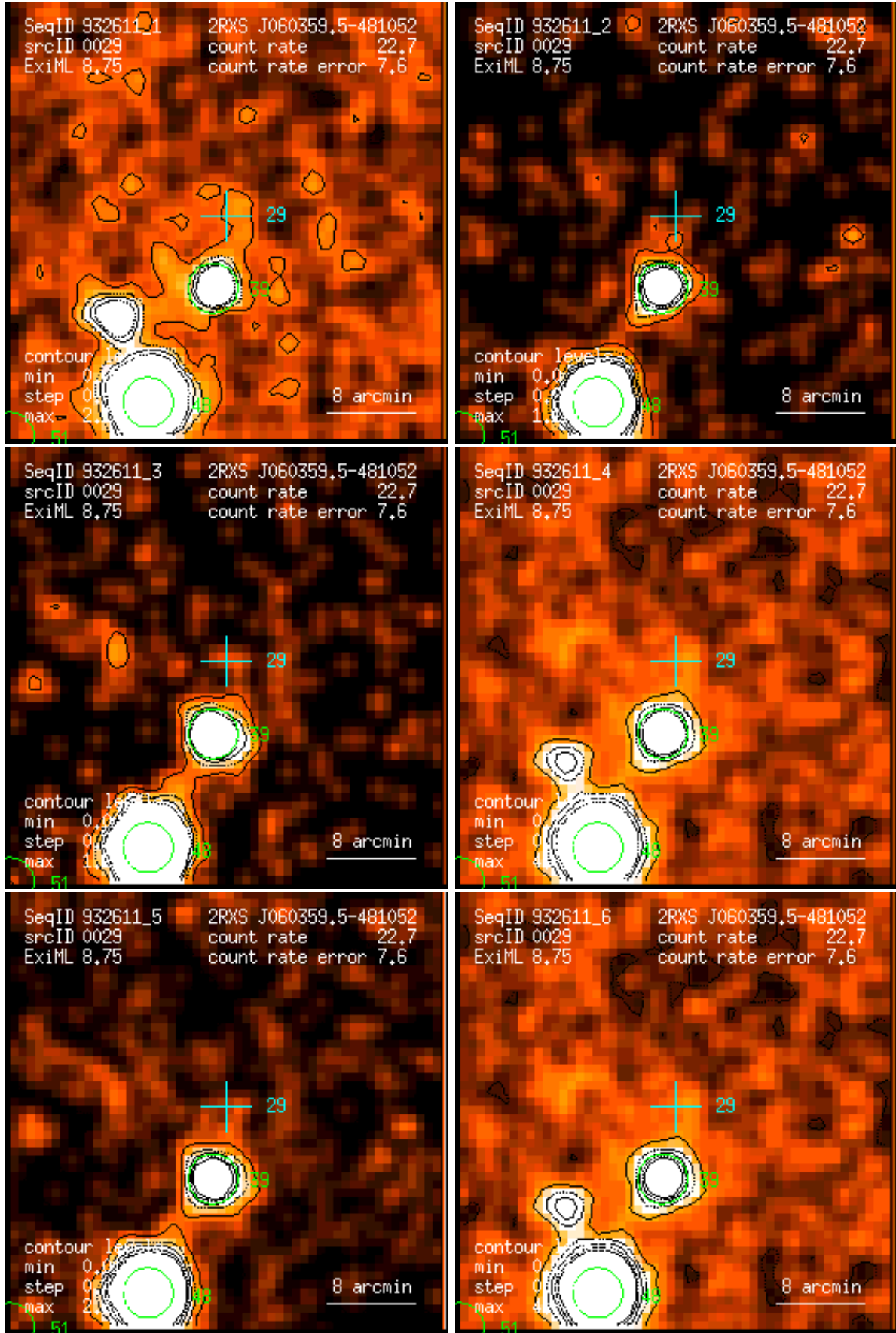
Figure 29: RASS 932611: detection 0029: band rate images, Gaussian filter: (1) PSPC channels 11 – 41, (2) 52 – 90, (3) 91 – 201, (4) 11 – 235, (5) 52 – 201, (6) 11 – 201. Broad band rates in counts/ks. Band rate contour levels in counts/ks/arcmin 2 .
