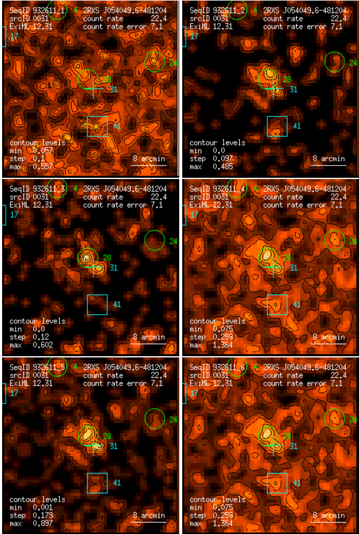
Figure 31: RASS 932611: detection 0031: band rate images, Gaussian filter: (1) PSPC channels 11 – 41, (2) 52 – 90, (3) 91 – 201, (4) 11 – 235, (5) 52 – 201, (6) 11 – 201. Broad band rates in counts/ks. Band rate contour levels in counts/ks/arcmin 2 .
