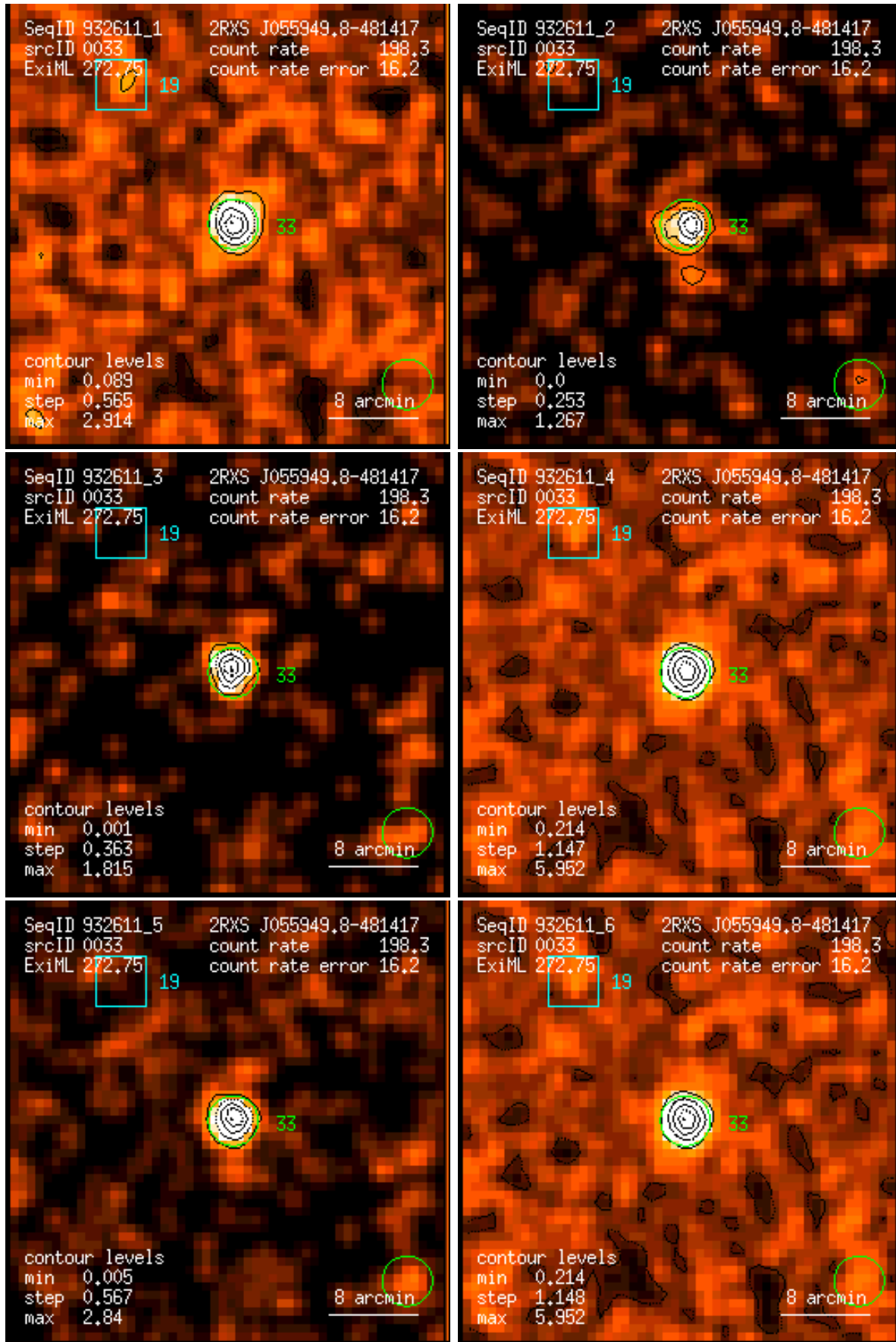
Figure 33: RASS 932611: detection 0033: band rate images, Gaussian filter: (1) PSPC channels 11 – 41, (2) 52 – 90, (3) 91 – 201, (4) 11 – 235, (5) 52 – 201, (6) 11 – 201. Broad band rates in counts/ks. Band rate contour levels in counts/ks/arcmin 2 .
