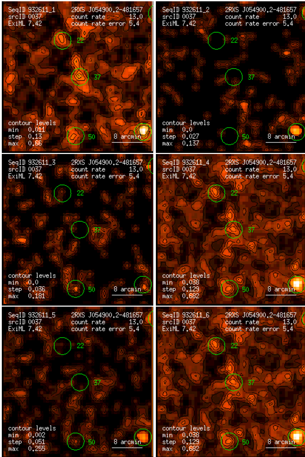
Figure 37: RASS 932611: detection 0037: band rate images, Gaussian filter: (1) PSPC channels 11 – 41, (2) 52 – 90, (3) 91 – 201, (4) 11 – 235, (5) 52 – 201, (6) 11 – 201. Broad band rates in counts/ks. Band rate contour levels in counts/ks/arcmin 2 .
