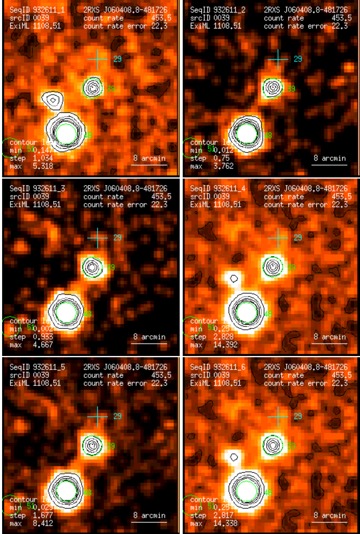
Figure 39: RASS 932611: detection 0039: band rate images, Gaussian filter: (1) PSPC channels 11 – 41, (2) 52 – 90, (3) 91 – 201, (4) 11 – 235, (5) 52 – 201, (6) 11 – 201. Broad band rates in counts/ks. Band rate contour levels in counts/ks/arcmin 2 .
