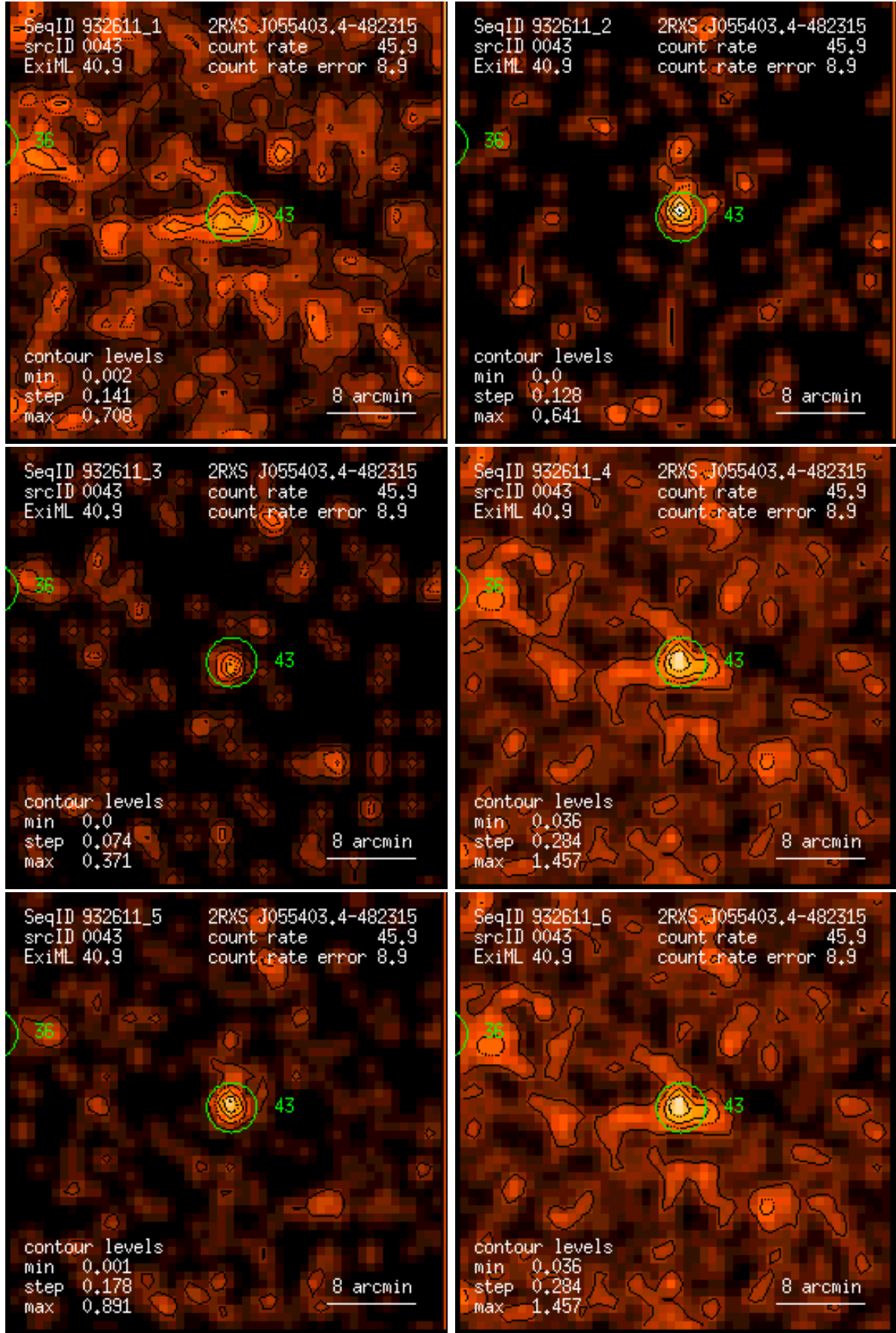
Figure 43: RASS 932611: detection 0043: band rate images, Gaussian filter: (1) PSPC channels 11 – 41, (2) 52 – 90, (3) 91 – 201, (4) 11 – 235, (5) 52 – 201, (6) 11 – 201. Broad band rates in counts/ks. Band rate contour levels in counts/ks/arcmin 2 .
