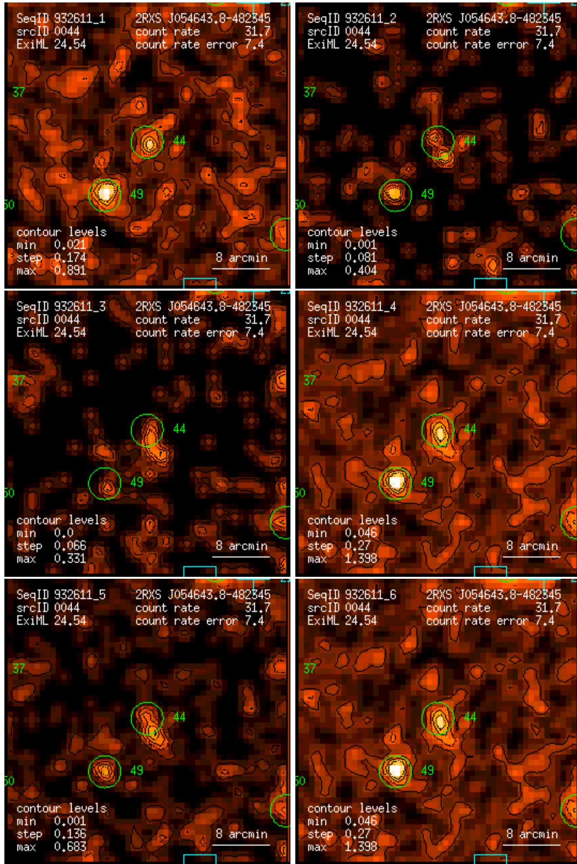
Figure 44: RASS 932611: detection 0044: band rate images, Gaussian filter: (1) PSPC channels 11 – 41, (2) 52 – 90, (3) 91 – 201, (4) 11 – 235, (5) 52 – 201, (6) 11 – 201. Broad band rates in counts/ks. Band rate contour levels in counts/ks/arcmin 2 .
