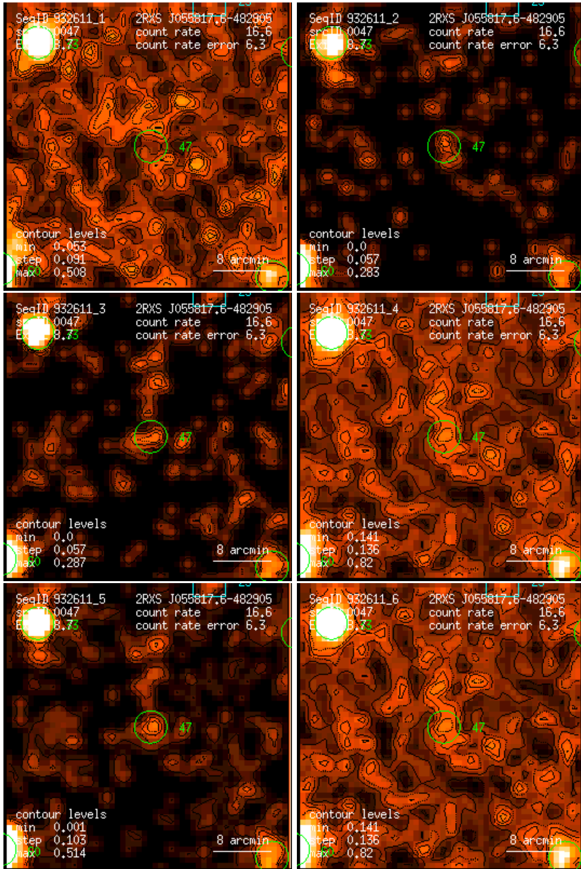
Figure 47: RASS 932611: detection 0047: band rate images, Gaussian filter: (1) PSPC channels 11 – 41, (2) 52 – 90, (3) 91 – 201, (4) 11 – 235, (5) 52 – 201, (6) 11 – 201. Broad band rates in counts/ks. Band rate contour levels in counts/ks/arcmin 2 .
