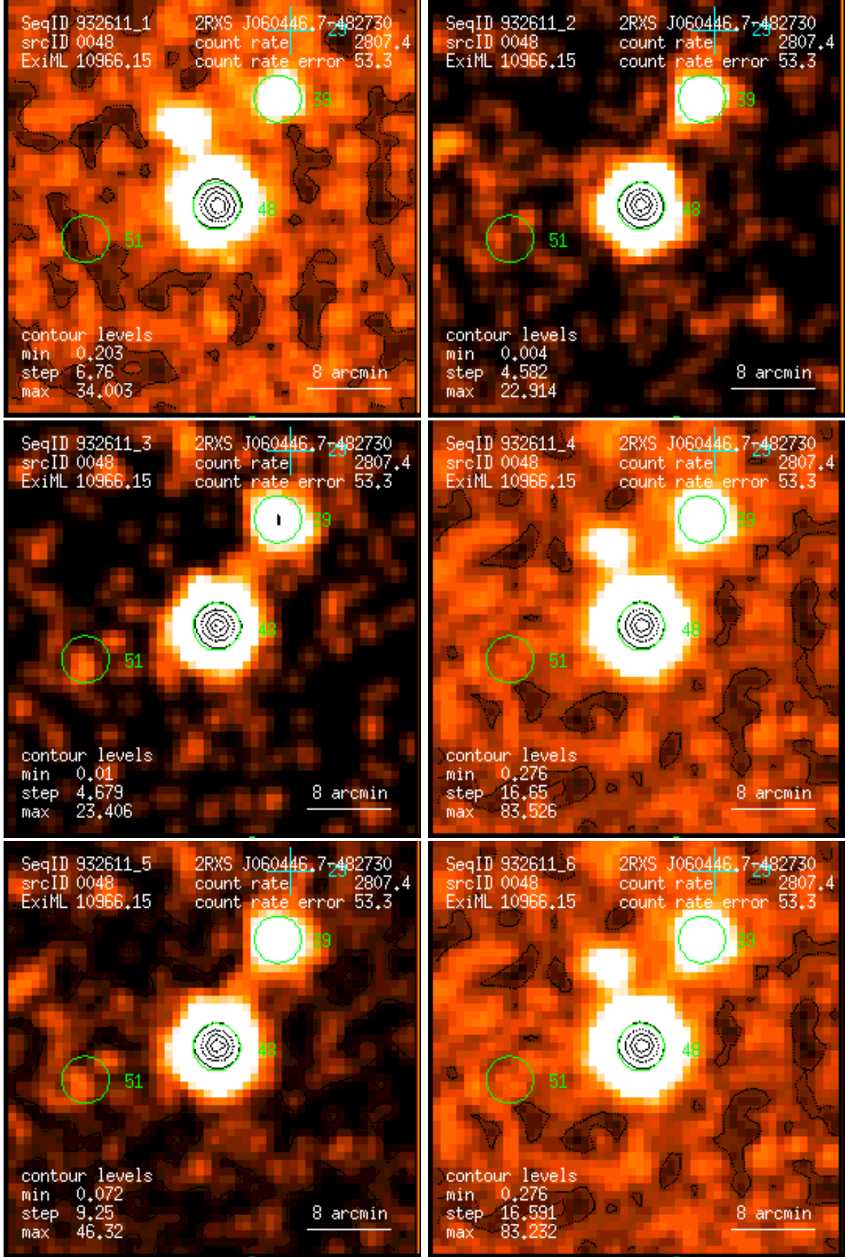
Figure 48: RASS 932611: detection 0048: band rate images, Gaussian filter: (1) PSPC channels 11 – 41, (2) 52 – 90, (3) 91 – 201, (4) 11 – 235, (5) 52 – 201, (6) 11 – 201. Broad band rates in counts/ks. Band rate contour levels in counts/ks/arcmin 2 .
