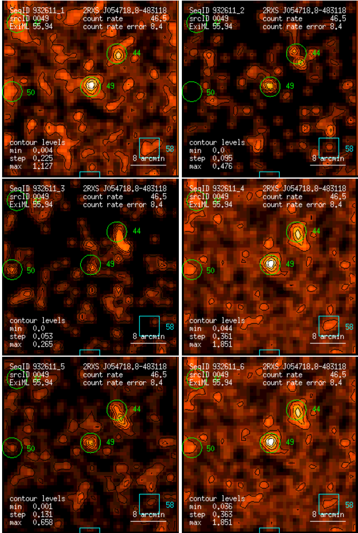
Figure 49: RASS 932611: detection 0049: band rate images, Gaussian filter: (1) PSPC channels 11 – 41, (2) 52 – 90, (3) 91 – 201, (4) 11 – 235, (5) 52 – 201, (6) 11 – 201. Broad band rates in counts/ks. Band rate contour levels in counts/ks/arcmin 2 .
