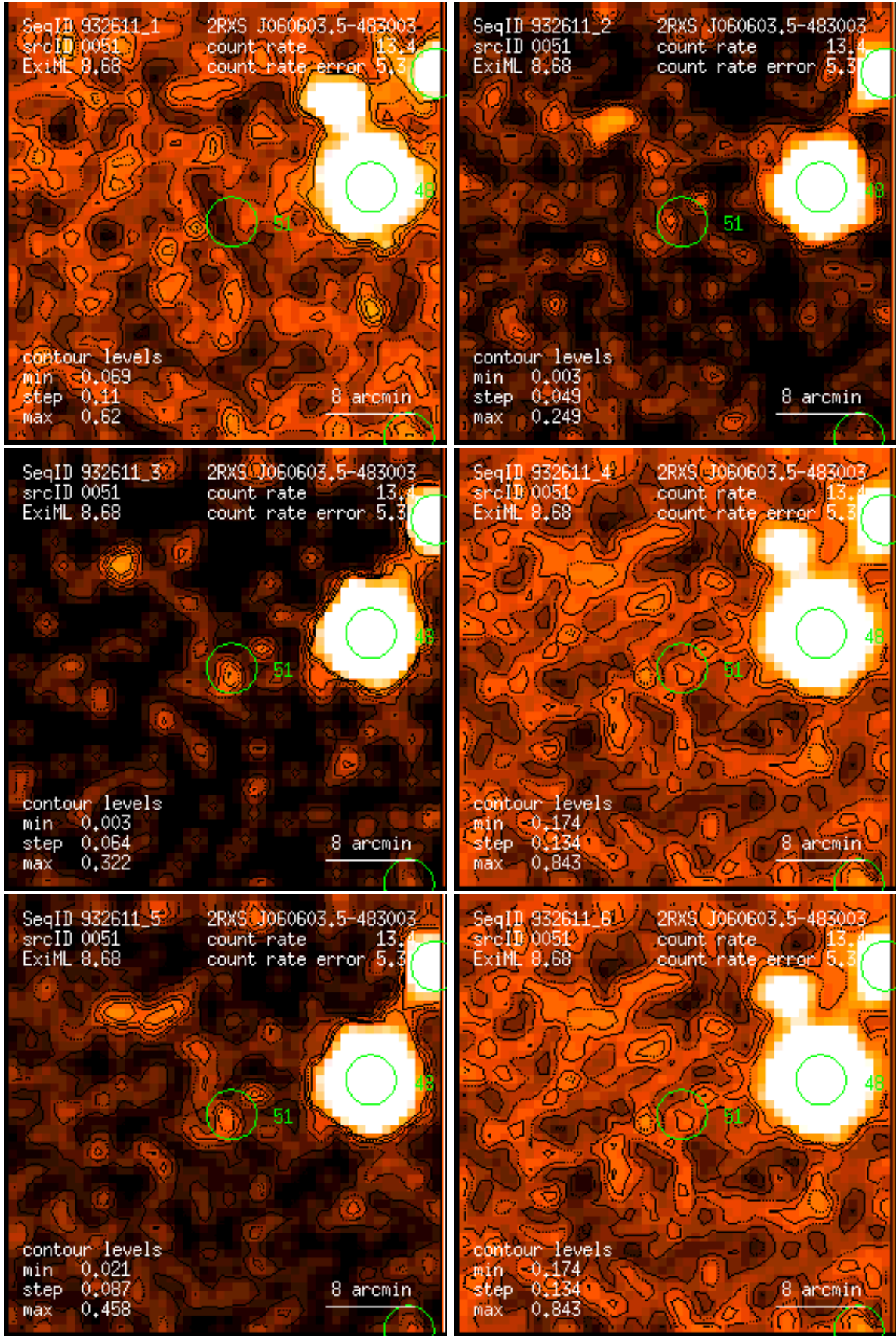
Figure 51: RASS 932611: detection 0051: band rate images, Gaussian filter: (1) PSPC channels 11 – 41, (2) 52 – 90, (3) 91 – 201, (4) 11 – 235, (5) 52 – 201, (6) 11 – 201. Broad band rates in counts/ks. Band rate contour levels in counts/ks/arcmin 2 .
