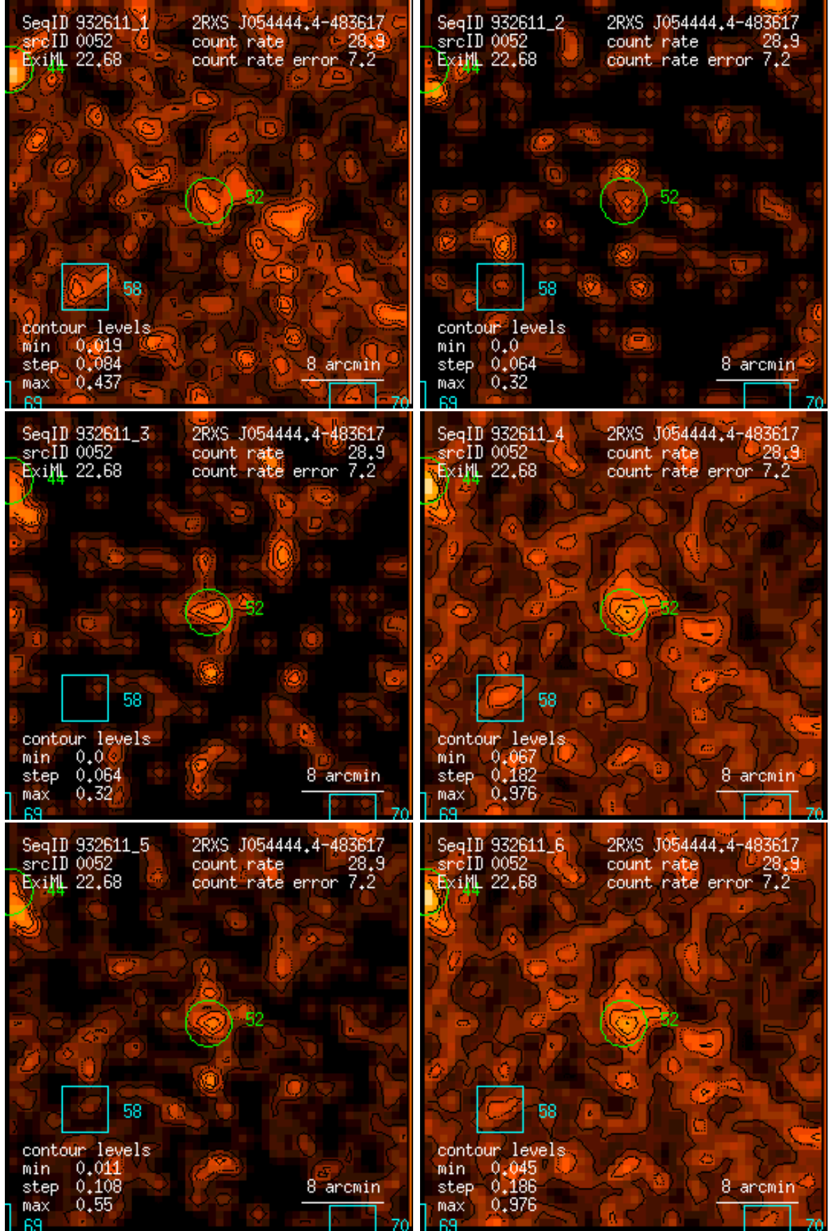
Figure 52: RASS 932611: detection 0052: band rate images, Gaussian filter: (1) PSPC channels 11 – 41, (2) 52 – 90, (3) 91 – 201, (4) 11 – 235, (5) 52 – 201, (6) 11 – 201. Broad band rates in counts/ks. Band rate contour levels in counts/ks/arcmin 2 .
