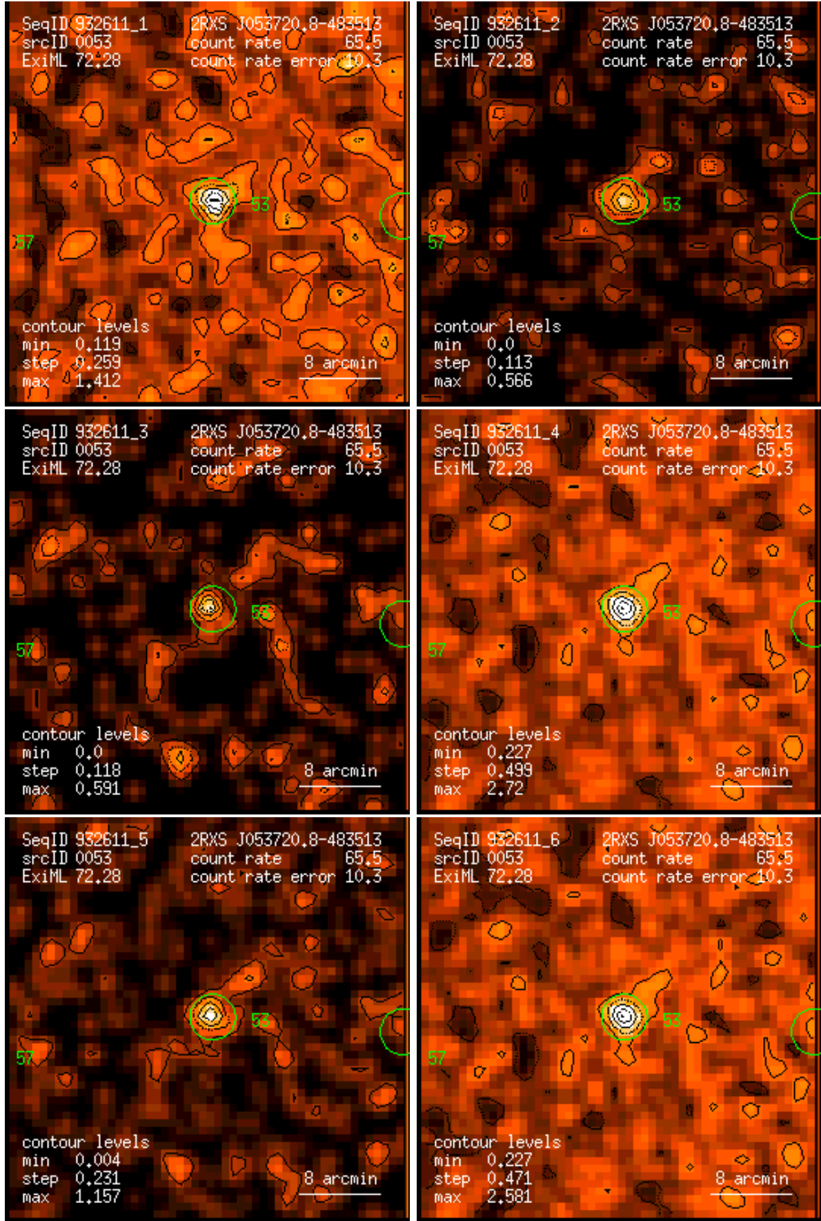
Figure 53: RASS 932611: detection 0053: band rate images, Gaussian filter: (1) PSPC channels 11 – 41, (2) 52 – 90, (3) 91 – 201, (4) 11 – 235, (5) 52 – 201, (6) 11 – 201. Broad band rates in counts/ks. Band rate contour levels in counts/ks/arcmin 2 .
