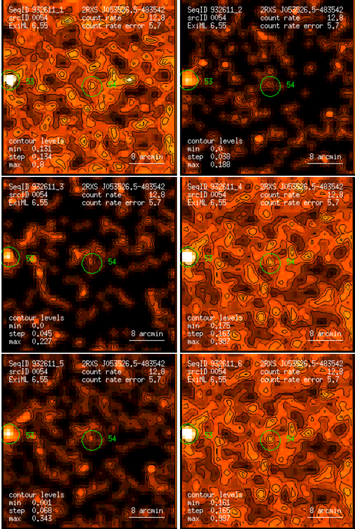
Figure 54: RASS 932611: detection 0054: band rate images, Gaussian filter: (1) PSPC channels 11 – 41, (2) 52 – 90, (3) 91 – 201, (4) 11 – 235, (5) 52 – 201, (6) 11 – 201. Broad band rates in counts/ks. Band rate contour levels in counts/ks/arcmin 2 .
