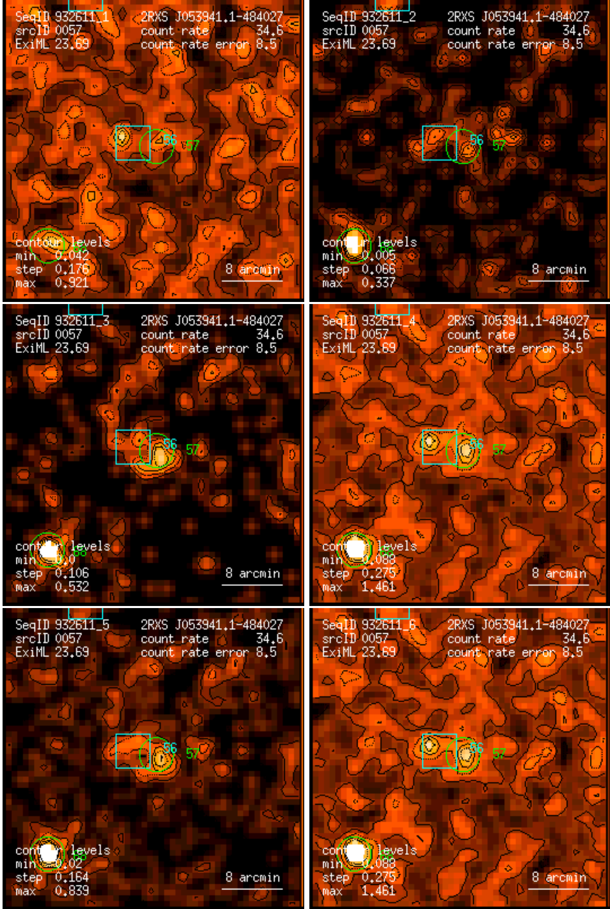
Figure 57: RASS 932611: detection 0057: band rate images, Gaussian filter: (1) PSPC channels 11 – 41, (2) 52 – 90, (3) 91 – 201, (4) 11 – 235, (5) 52 – 201, (6) 11 – 201. Broad band rates in counts/ks. Band rate contour levels in counts/ks/arcmin 2 .
