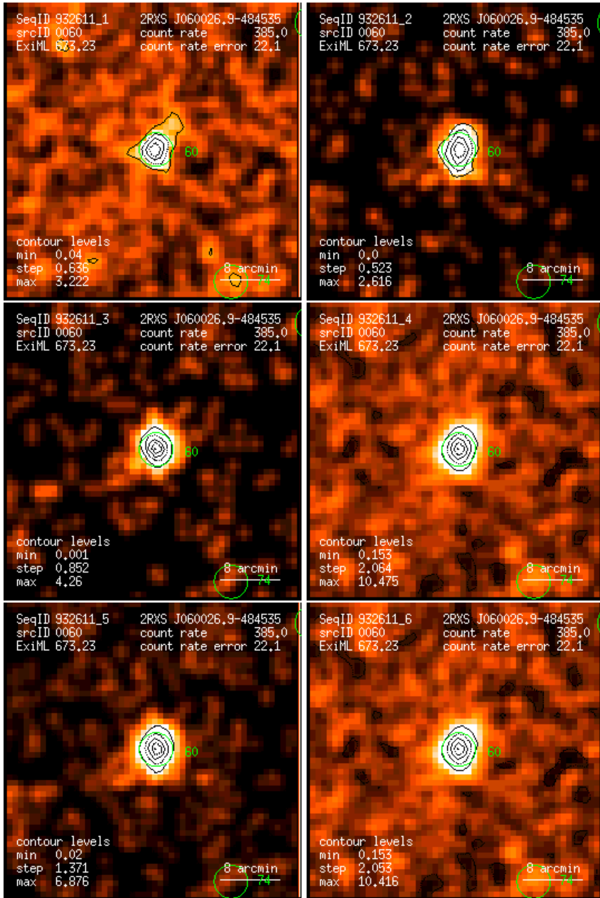
Figure 60: RASS 932611: detection 0060: band rate images, Gaussian filter: (1) PSPC channels 11 – 41, (2) 52 – 90, (3) 91 – 201, (4) 11 – 235, (5) 52 – 201, (6) 11 – 201. Broad band rates in counts/ks. Band rate contour levels in counts/ks/arcmin 2 .
