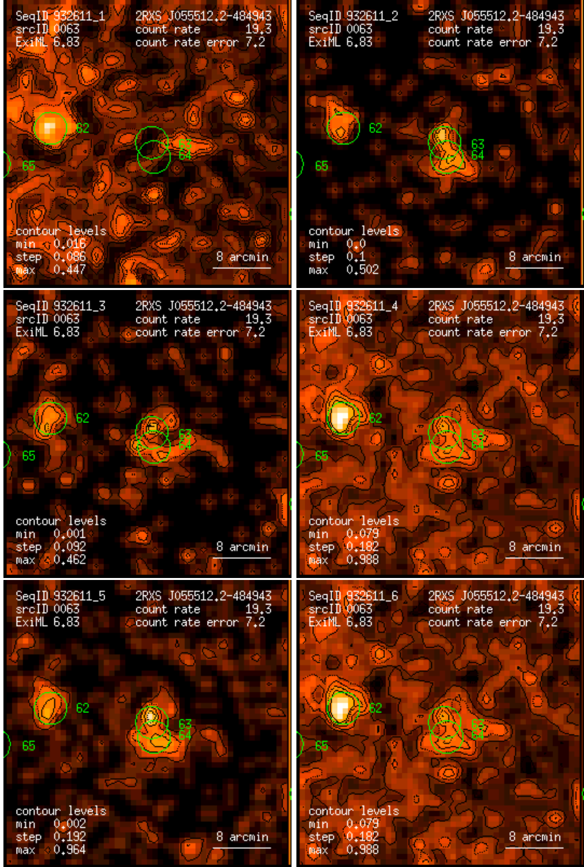
Figure 63: RASS 932611: detection 0063: band rate images, Gaussian filter: (1) PSPC channels 11 – 41, (2) 52 – 90, (3) 91 – 201, (4) 11 – 235, (5) 52 – 201, (6) 11 – 201. Broad band rates in counts/ks. Band rate contour levels in counts/ks/arcmin 2 .
