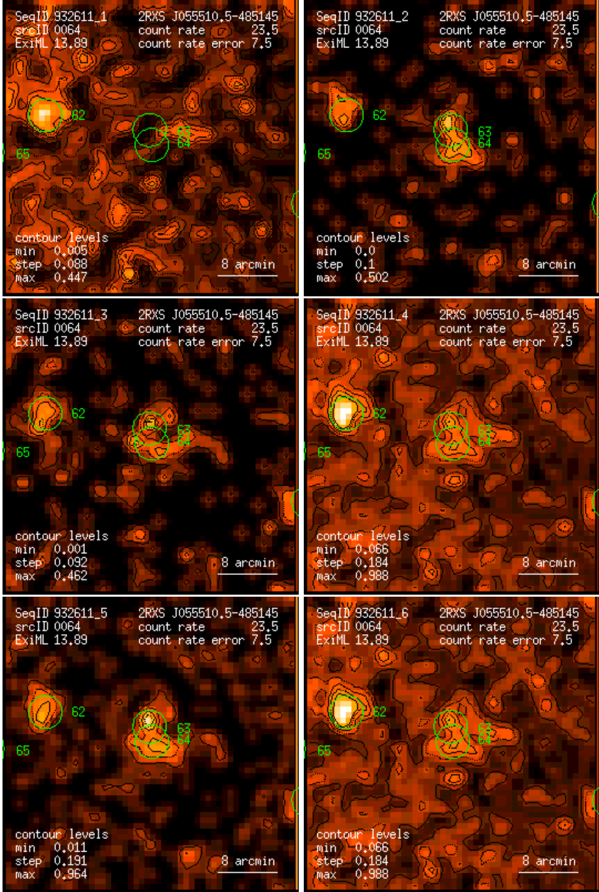
Figure 64: RASS 932611: detection 0064: band rate images, Gaussian filter: (1) PSPC channels 11 – 41, (2) 52 – 90, (3) 91 – 201, (4) 11 – 235, (5) 52 – 201, (6) 11 – 201. Broad band rates in counts/ks. Band rate contour levels in counts/ks/arcmin 2 .
