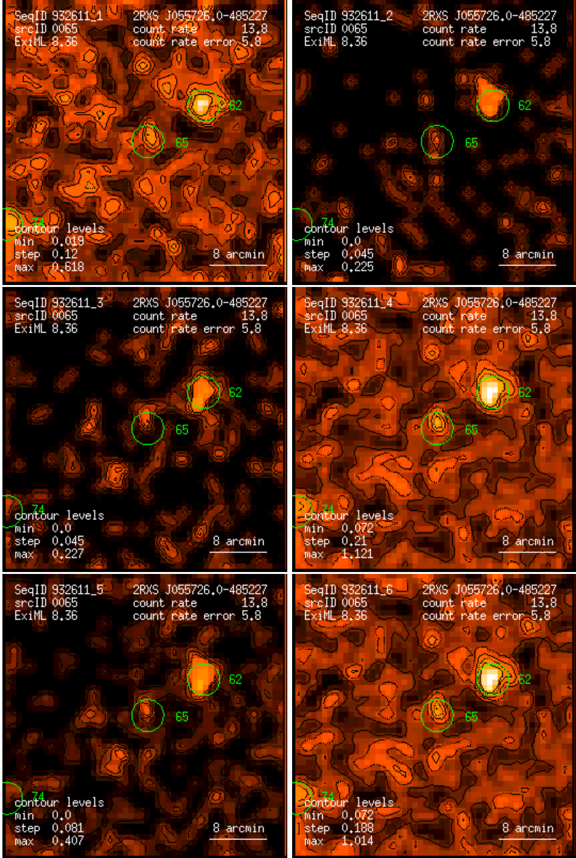
Figure 65: RASS 932611: detection 0065: band rate images, Gaussian filter: (1) PSPC channels 11 – 41, (2) 52 – 90, (3) 91 – 201, (4) 11 – 235, (5) 52 – 201, (6) 11 – 201. Broad band rates in counts/ks. Band rate contour levels in counts/ks/arcmin 2 .
