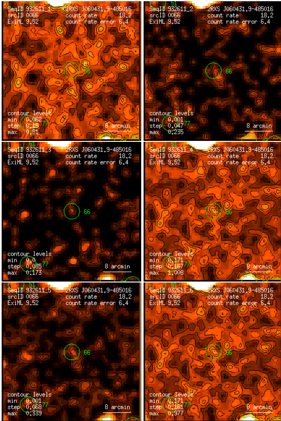
Figure 66: RASS 932611: detection 0066: band rate images, Gaussian filter: (1) PSPC channels 11 – 41, (2) 52 – 90, (3) 91 – 201, (4) 11 – 235, (5) 52 – 201, (6) 11 – 201. Broad band rates in counts/ks. Band rate contour levels in counts/ks/arcmin 2 .
