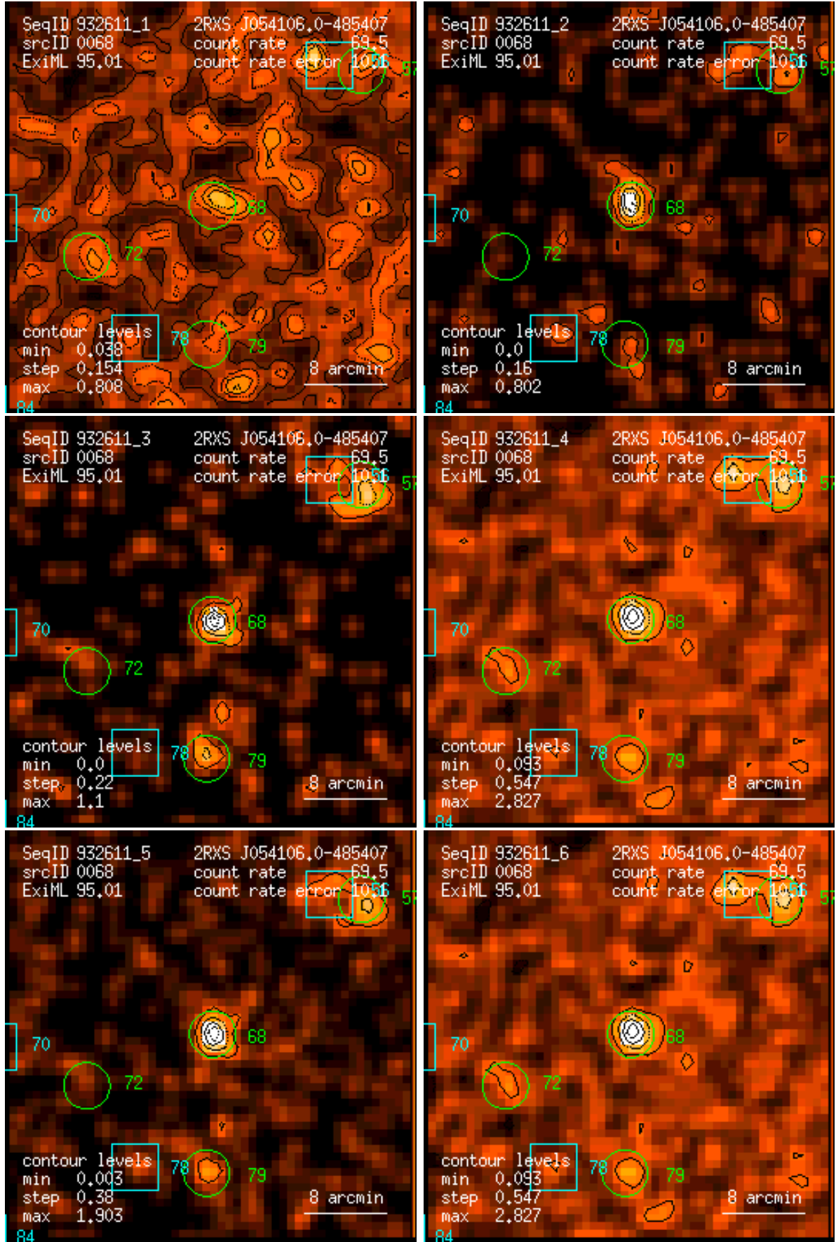
Figure 68: RASS 932611: detection 0068: band rate images, Gaussian filter: (1) PSPC channels 11 – 41, (2) 52 – 90, (3) 91 – 201, (4) 11 – 235, (5) 52 – 201, (6) 11 – 201. Broad band rates in counts/ks. Band rate contour levels in counts/ks/arcmin 2 .
