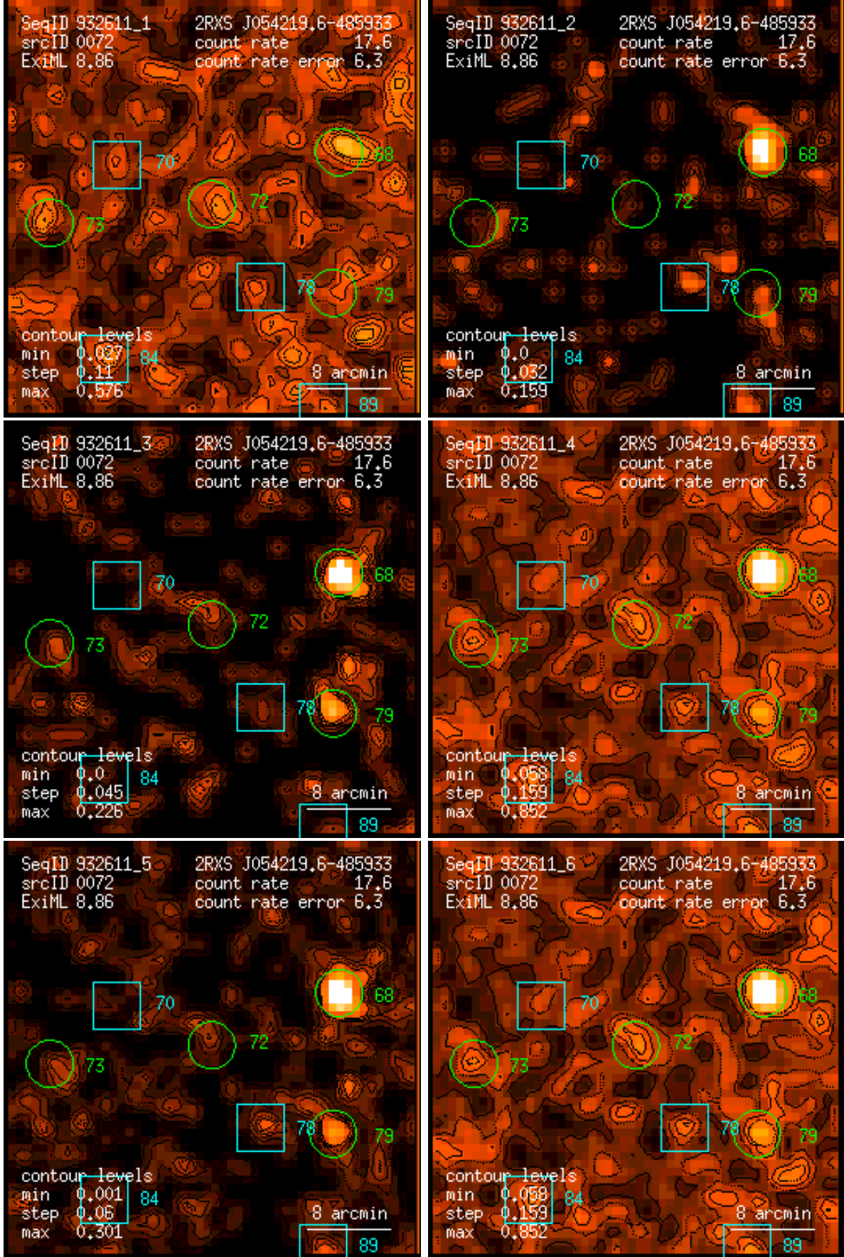
Figure 72: RASS 932611: detection 0072: band rate images, Gaussian filter: (1) PSPC channels 11 – 41, (2) 52 – 90, (3) 91 – 201, (4) 11 – 235, (5) 52 – 201, (6) 11 – 201. Broad band rates in counts/ks. Band rate contour levels in counts/ks/arcmin 2 .
