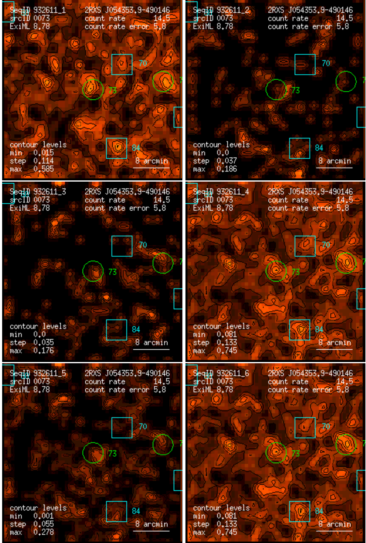
Figure 73: RASS 932611: detection 0073: band rate images, Gaussian filter: (1) PSPC channels 11 – 41, (2) 52 – 90, (3) 91 – 201, (4) 11 – 235, (5) 52 – 201, (6) 11 – 201. Broad band rates in counts/ks. Band rate contour levels in counts/ks/arcmin 2 .
