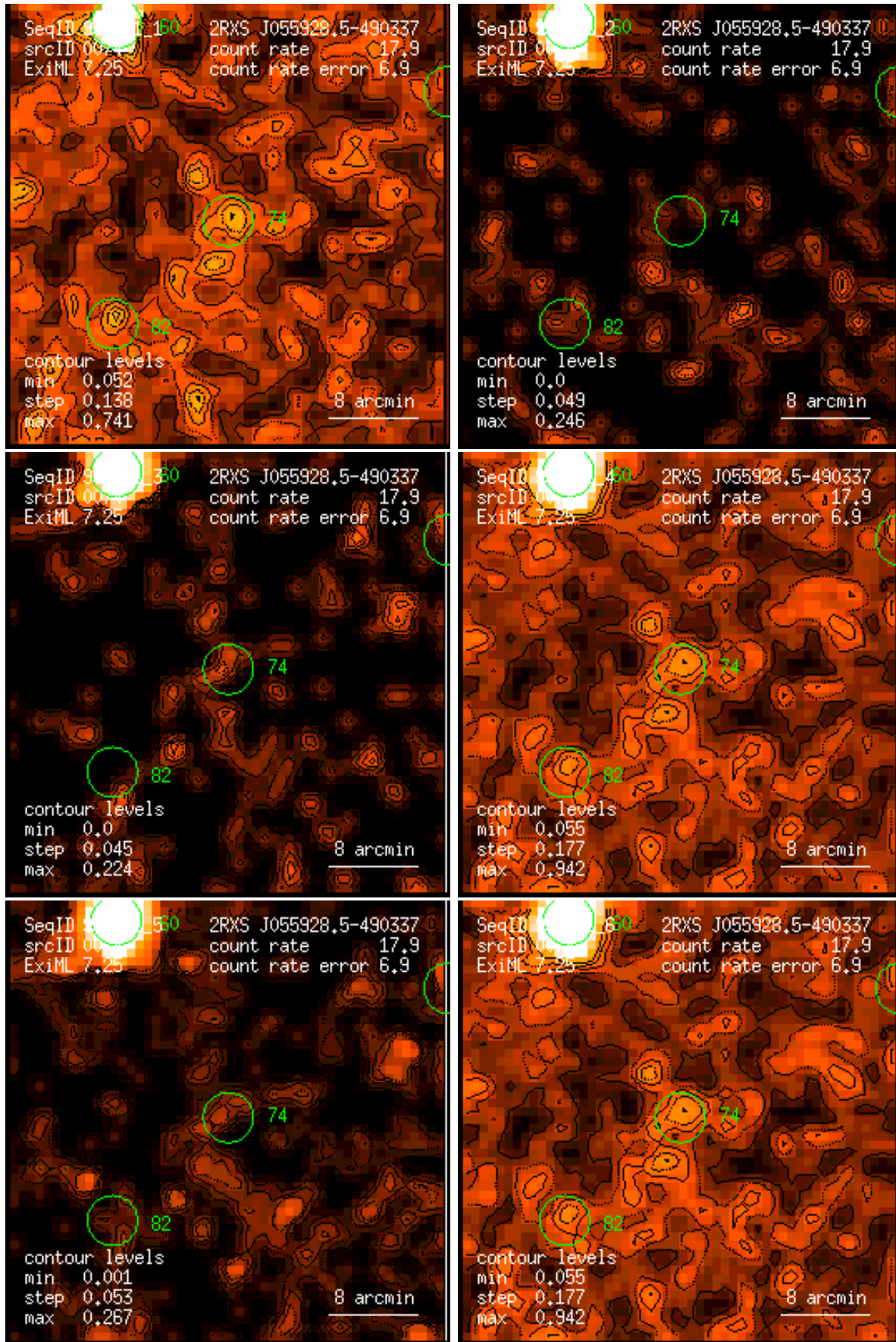
Figure 74: RASS 932611: detection 0074: band rate images, Gaussian filter: (1) PSPC channels 11 – 41, (2) 52 – 90, (3) 91 – 201, (4) 11 – 235, (5) 52 – 201, (6) 11 – 201. Broad band rates in counts/ks. Band rate contour levels in counts/ks/arcmin 2 .
