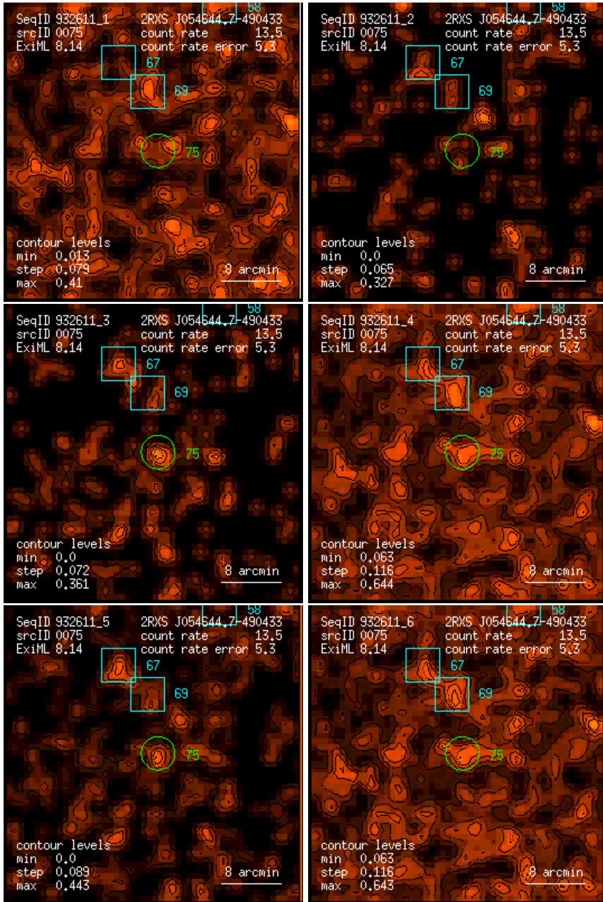
Figure 75: RASS 932611: detection 0075: band rate images, Gaussian filter: (1) PSPC channels 11 – 41, (2) 52 – 90, (3) 91 – 201, (4) 11 – 235, (5) 52 – 201, (6) 11 – 201. Broad band rates in counts/ks. Band rate contour levels in counts/ks/arcmin 2 .
