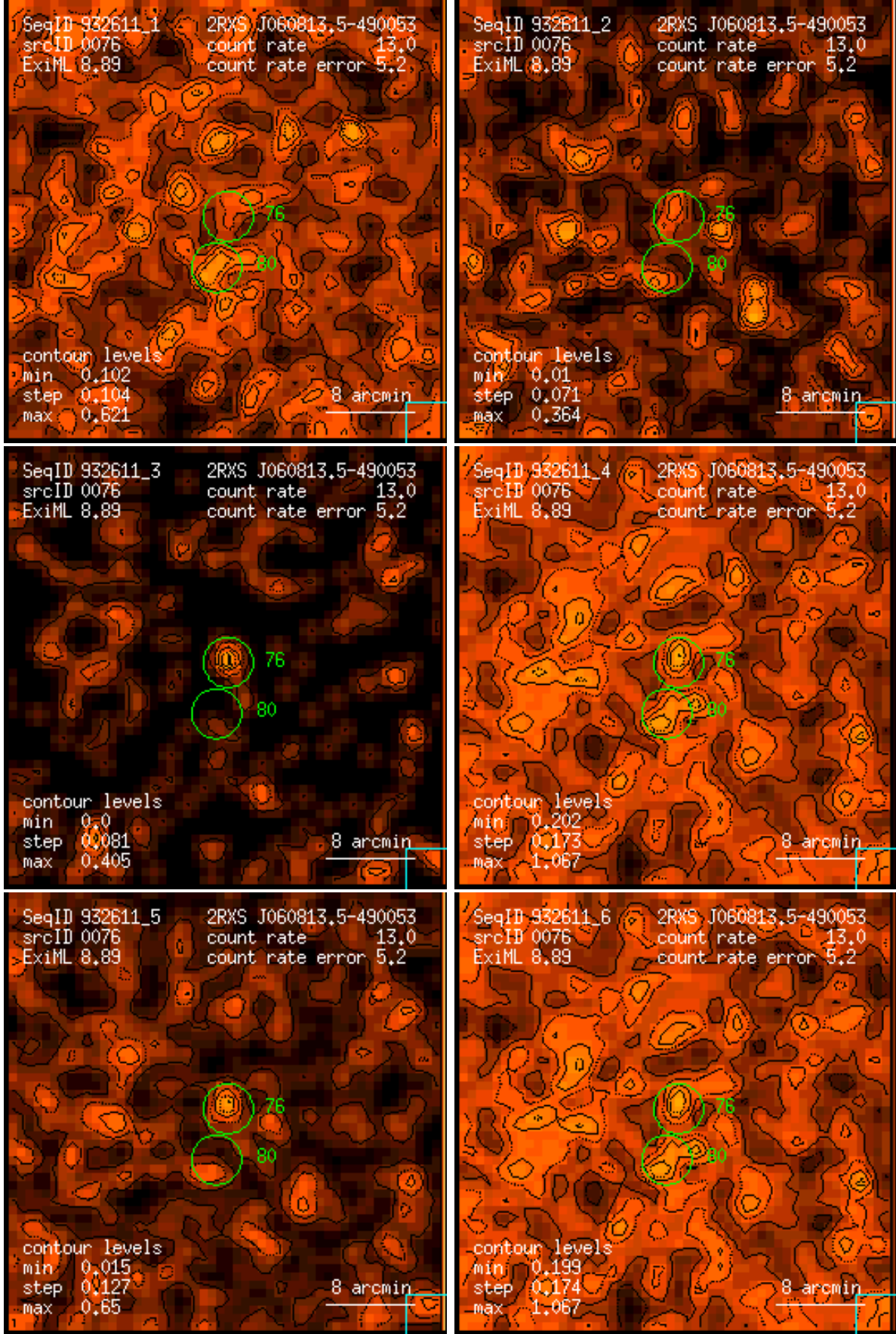
Figure 76: RASS 932611: detection 0076: band rate images, Gaussian filter: (1) PSPC channels 11 – 41, (2) 52 – 90, (3) 91 – 201, (4) 11 – 235, (5) 52 – 201, (6) 11 – 201. Broad band rates in counts/ks. Band rate contour levels in counts/ks/arcmin 2 .
