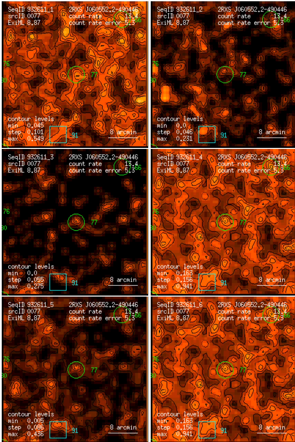
Figure 77: RASS 932611: detection 0077: band rate images, Gaussian filter: (1) PSPC channels 11 – 41, (2) 52 – 90, (3) 91 – 201, (4) 11 – 235, (5) 52 – 201, (6) 11 – 201. Broad band rates in counts/ks. Band rate contour levels in counts/ks/arcmin 2 .
